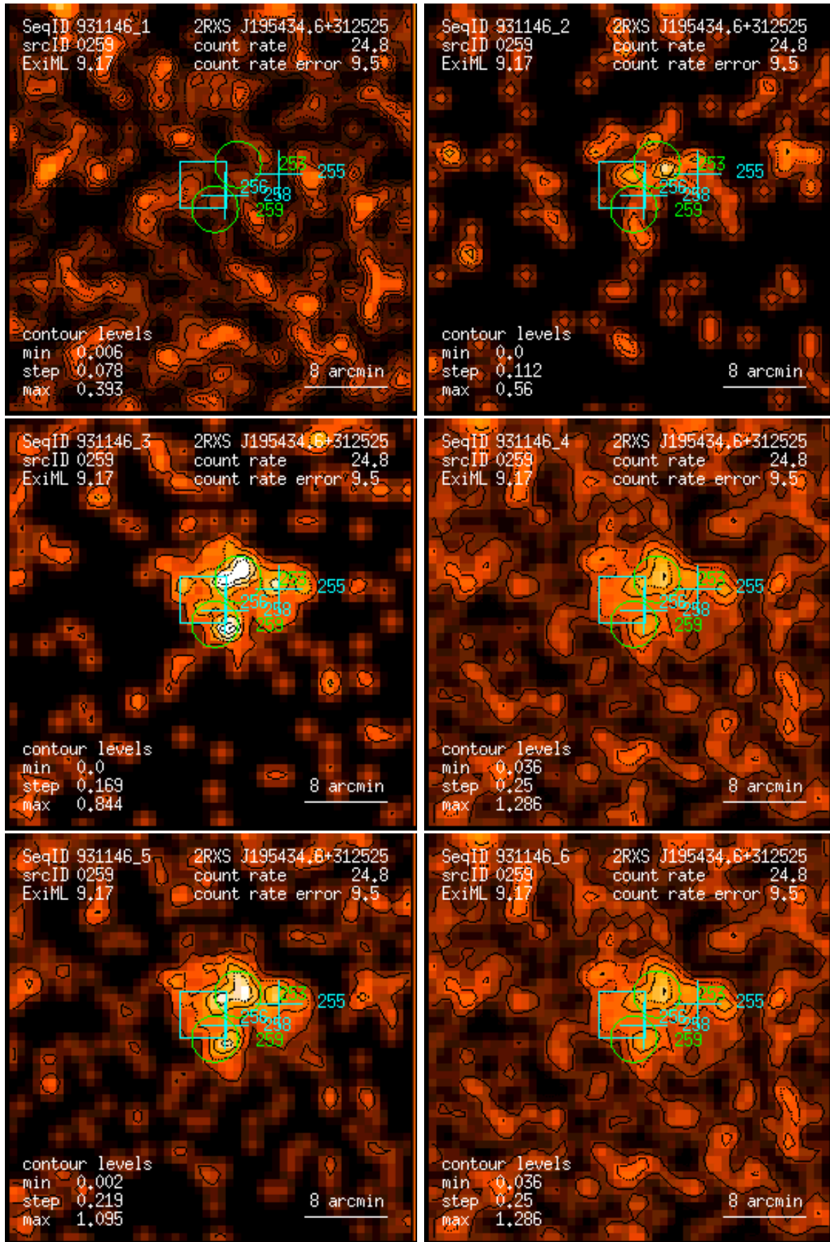
Figure 259: RASS 931146: detection 0259: band rate images, Gaussian filter: (1) PSPC channels 11 – 41, (2) 52 – 90, (3) 91 – 201, (4) 11 – 235, (5) 52 – 201, (6) 11 – 201. Broad band rates in counts/ks. Band rate contour levels in counts/ks/arcmin 2 .
