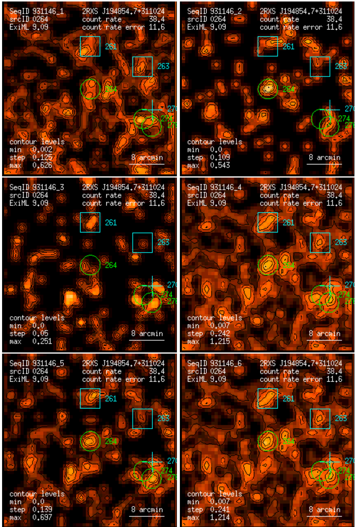
Figure 264: RASS 931146: detection 0264: band rate images, Gaussian filter: (1) PSPC channels 11 – 41, (2) 52 – 90, (3) 91 – 201, (4) 11 – 235, (5) 52 – 201, (6) 11 – 201. Broad band rates in counts/ks. Band rate contour levels in counts/ks/arcmin 2 .
