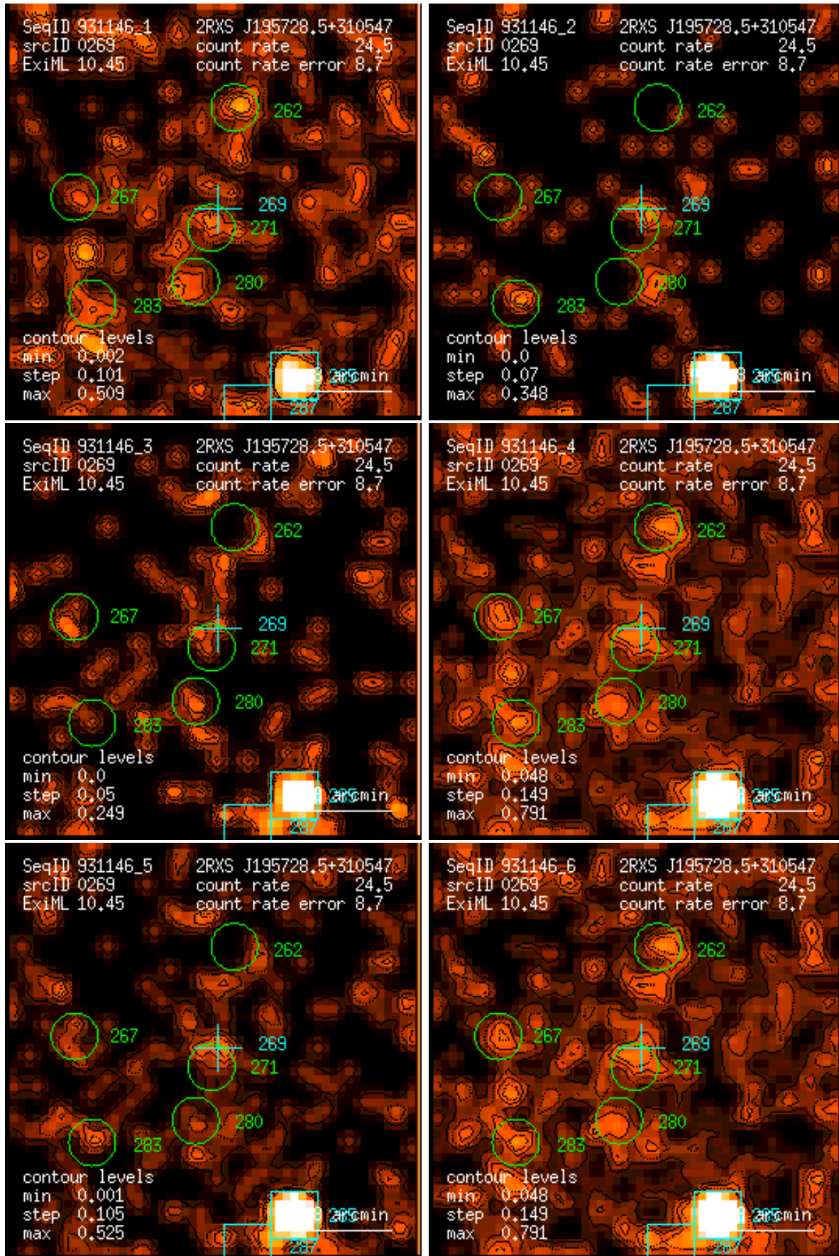
Figure 269: RASS 931146: detection 0269: band rate images, Gaussian filter: (1) PSPC channels 11 – 41, (2) 52 – 90, (3) 91 – 201, (4) 11 – 235, (5) 52 – 201, (6) 11 – 201. Broad band rates in counts/ks. Band rate contour levels in counts/ks/arcmin 2 .
