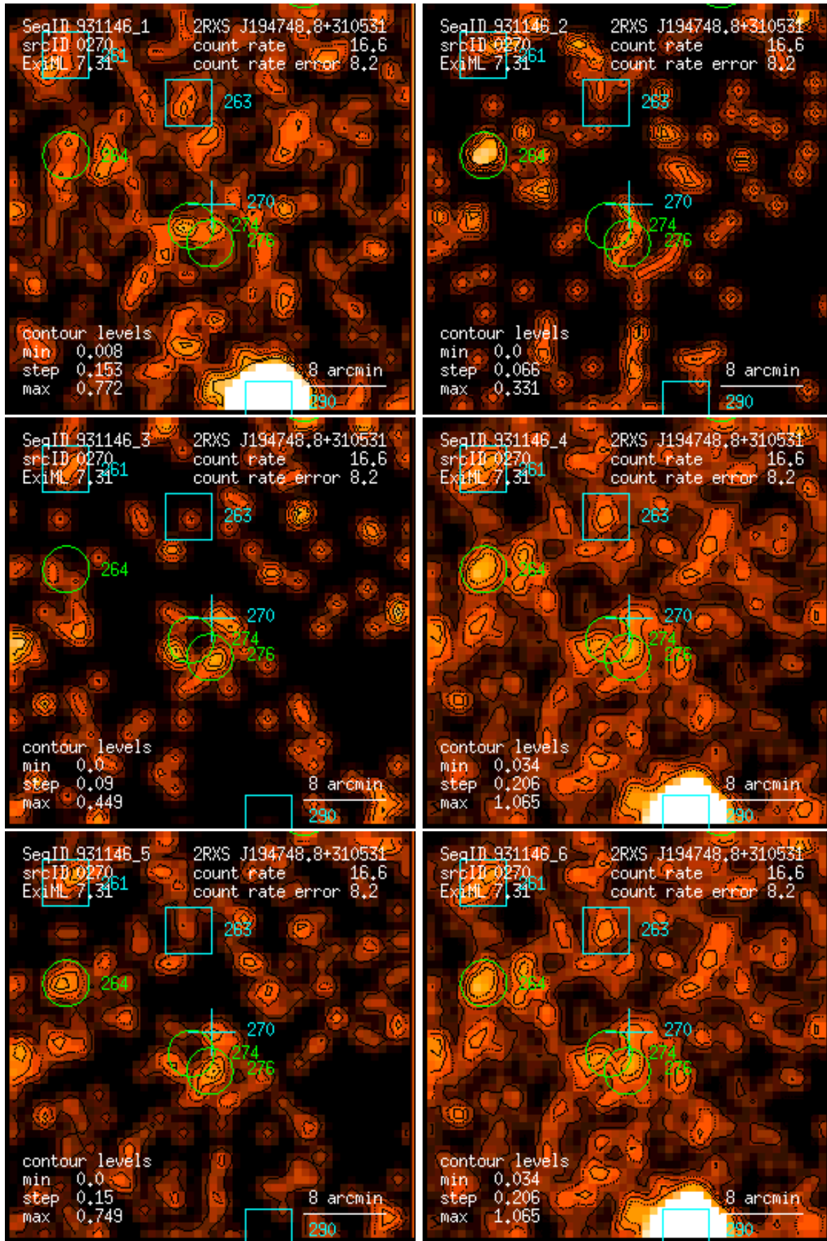
Figure 270: RASS 931146: detection 0270: band rate images, Gaussian filter: (1) PSPC channels 11 – 41, (2) 52 – 90, (3) 91 – 201, (4) 11 – 235, (5) 52 – 201, (6) 11 – 201. Broad band rates in counts/ks. Band rate contour levels in counts/ks/arcmin 2 .
