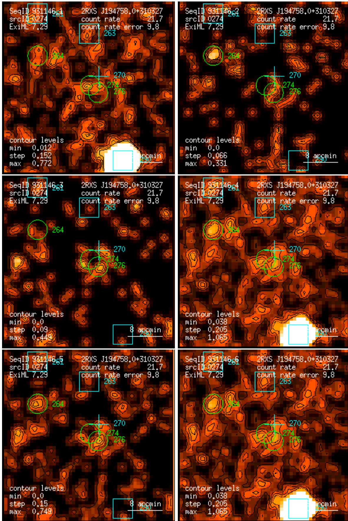
Figure 274: RASS 931146: detection 0274: band rate images, Gaussian filter: (1) PSPC channels 11 – 41, (2) 52 – 90, (3) 91 – 201, (4) 11 – 235, (5) 52 – 201, (6) 11 – 201. Broad band rates in counts/ks. Band rate contour levels in counts/ks/arcmin 2 .
