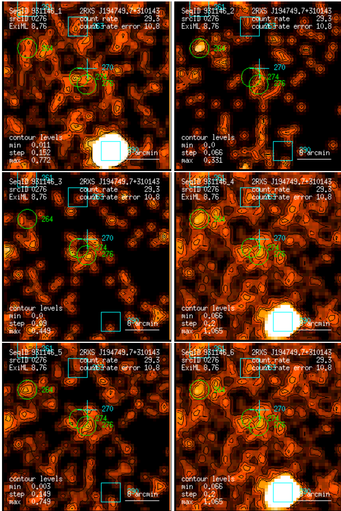
Figure 276: RASS 931146: detection 0276: band rate images, Gaussian filter: (1) PSPC channels 11 – 41, (2) 52 – 90, (3) 91 – 201, (4) 11 – 235, (5) 52 – 201, (6) 11 – 201. Broad band rates in counts/ks. Band rate contour levels in counts/ks/arcmin 2 .
