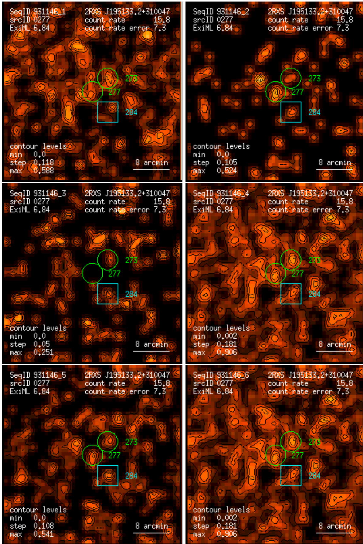
Figure 277: RASS 931146: detection 0277: band rate images, Gaussian filter: (1) PSPC channels 11 – 41, (2) 52 – 90, (3) 91 – 201, (4) 11 – 235, (5) 52 – 201, (6) 11 – 201. Broad band rates in counts/ks. Band rate contour levels in counts/ks/arcmin 2 .
