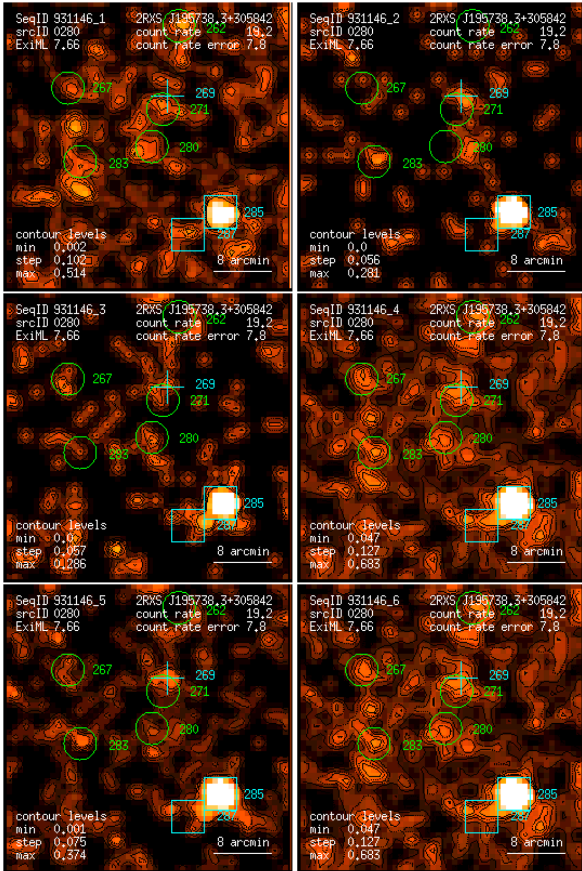
Figure 280: RASS 931146: detection 0280: band rate images, Gaussian filter: (1) PSPC channels 11 – 41, (2) 52 – 90, (3) 91 – 201, (4) 11 – 235, (5) 52 – 201, (6) 11 – 201. Broad band rates in counts/ks. Band rate contour levels in counts/ks/arcmin 2 .
