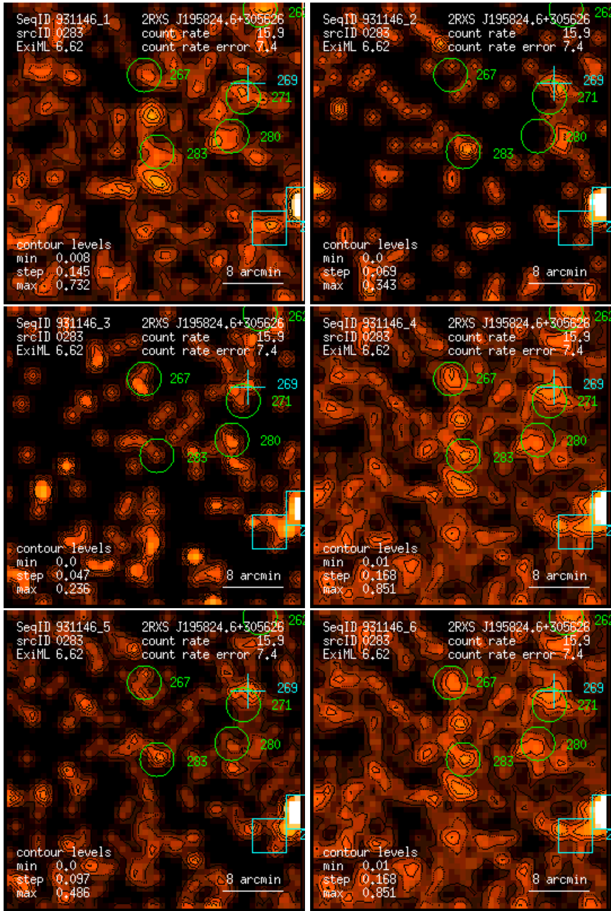
Figure 283: RASS 931146: detection 0283: band rate images, Gaussian filter: (1) PSPC channels 11 – 41, (2) 52 – 90, (3) 91 – 201, (4) 11 – 235, (5) 52 – 201, (6) 11 – 201. Broad band rates in counts/ks. Band rate contour levels in counts/ks/arcmin 2 .
