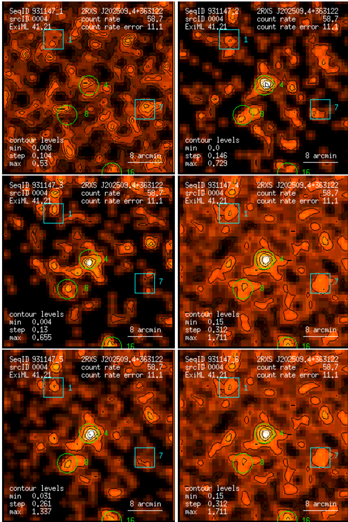
Figure 4: RASS 931147: detection 0004: band rate images, Gaussian filter: (1) PSPC channels 11 – 41, (2) 52 – 90, (3) 91 – 201, (4) 11 – 235, (5) 52 – 201, (6) 11 – 201. Broad band rates in counts/ks. Band rate contour levels in counts/ks/arcmin 2 .
