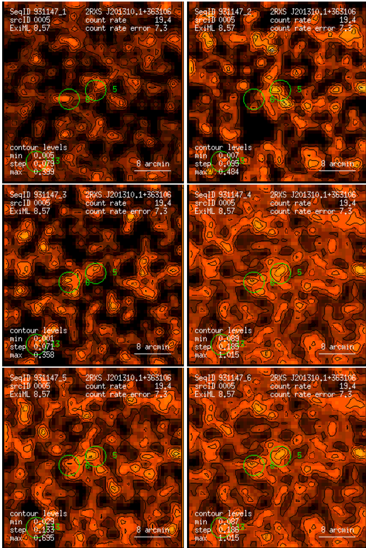
Figure 5: RASS 931147: detection 0005: band rate images, Gaussian filter: (1) PSPC channels 11 – 41, (2) 52 – 90, (3) 91 – 201, (4) 11 – 235, (5) 52 – 201, (6) 11 – 201. Broad band rates in counts/ks. Band rate contour levels in counts/ks/arcmin 2 .
