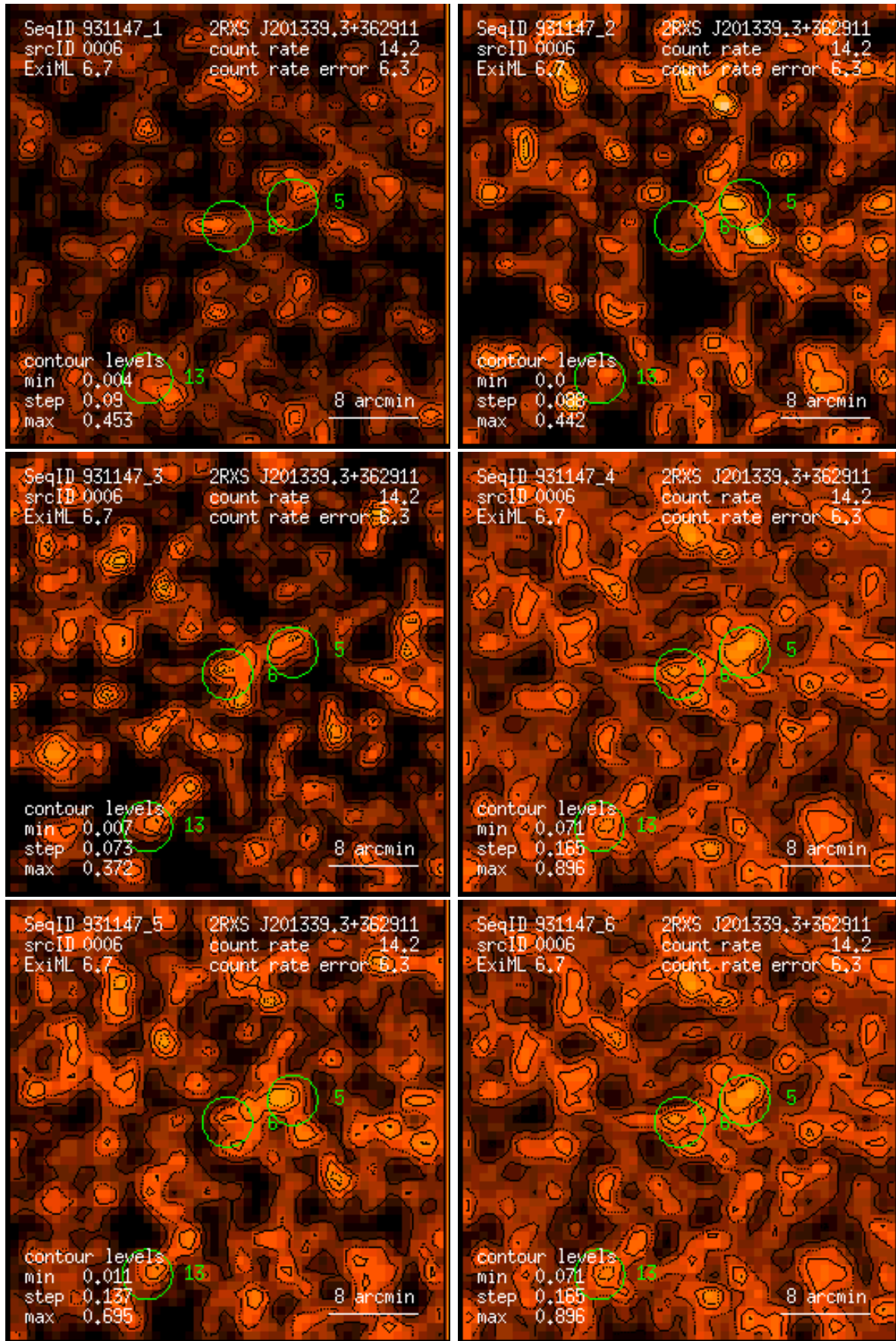
Figure 6: RASS 931147: detection 0006: band rate images, Gaussian filter: (1) PSPC channels 11 – 41, (2) 52 – 90, (3) 91 – 201, (4) 11 – 235, (5) 52 – 201, (6) 11 – 201. Broad band rates in counts/ks. Band rate contour levels in counts/ks/arcmin 2 .
