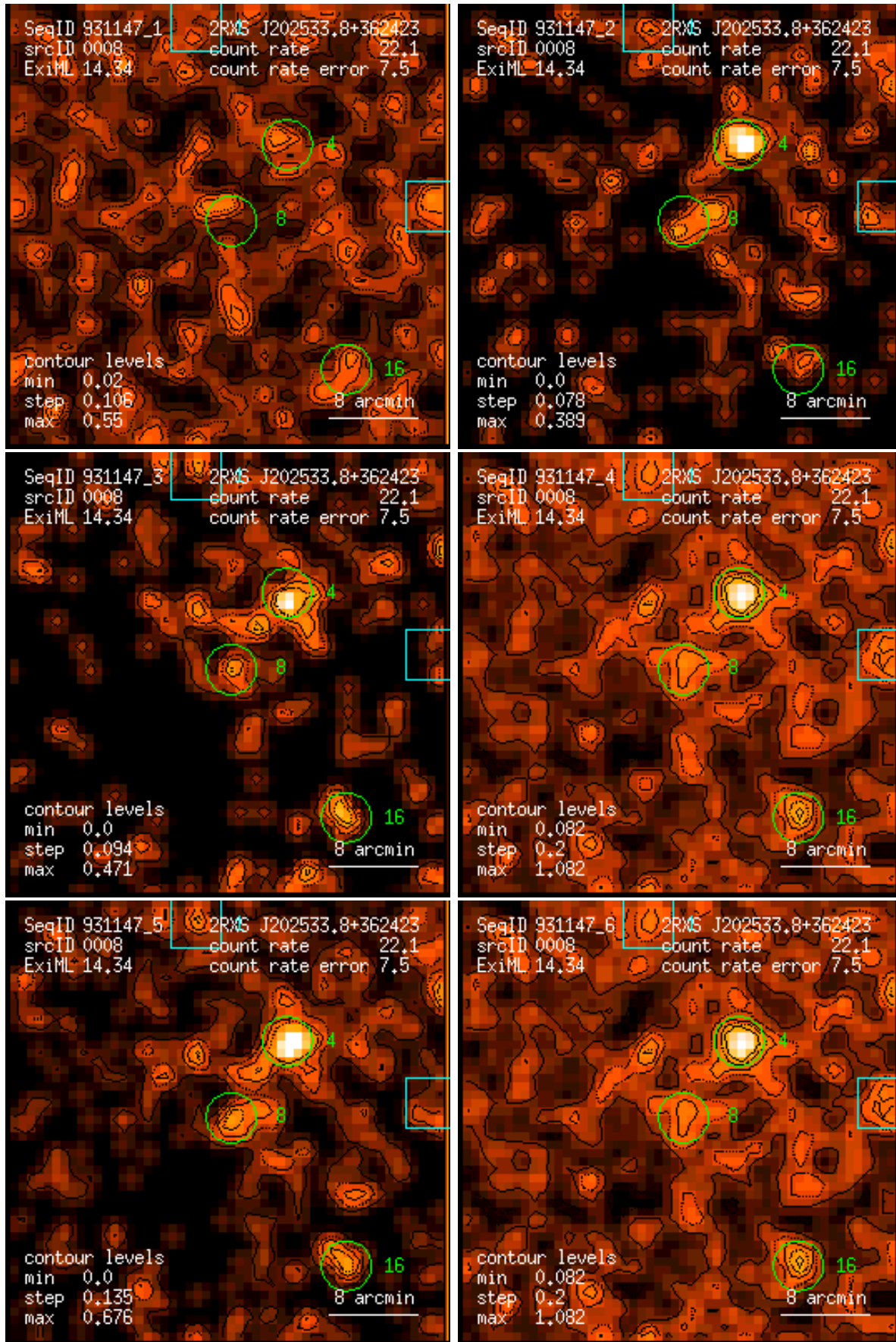
Figure 8: RASS 931147: detection 0008: band rate images, Gaussian filter: (1) PSPC channels 11 – 41, (2) 52 – 90, (3) 91 – 201, (4) 11 – 235, (5) 52 – 201, (6) 11 – 201. Broad band rates in counts/ks. Band rate contour levels in counts/ks/arcmin 2 .
