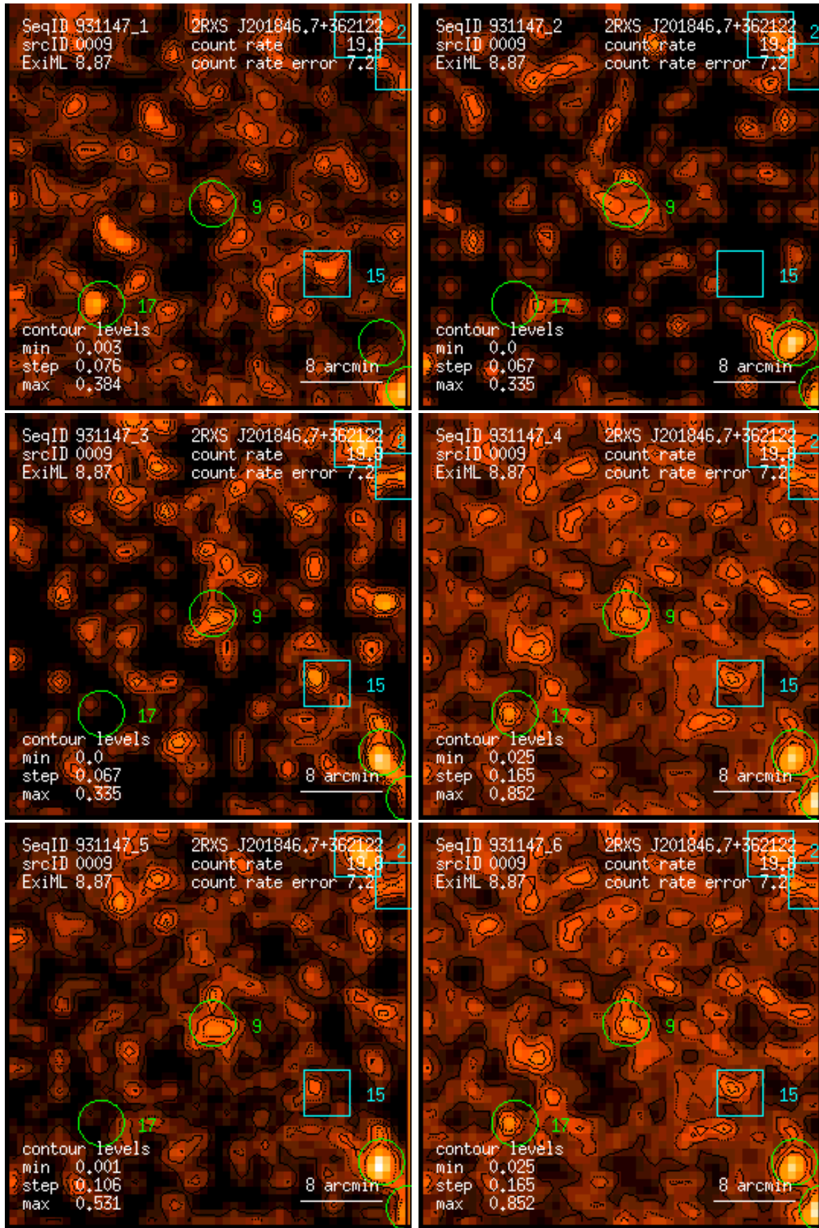
Figure 9: RASS 931147: detection 0009: band rate images, Gaussian filter: (1) PSPC channels 11 – 41, (2) 52 – 90, (3) 91 – 201, (4) 11 – 235, (5) 52 – 201, (6) 11 – 201. Broad band rates in counts/ks. Band rate contour levels in counts/ks/arcmin 2 .
