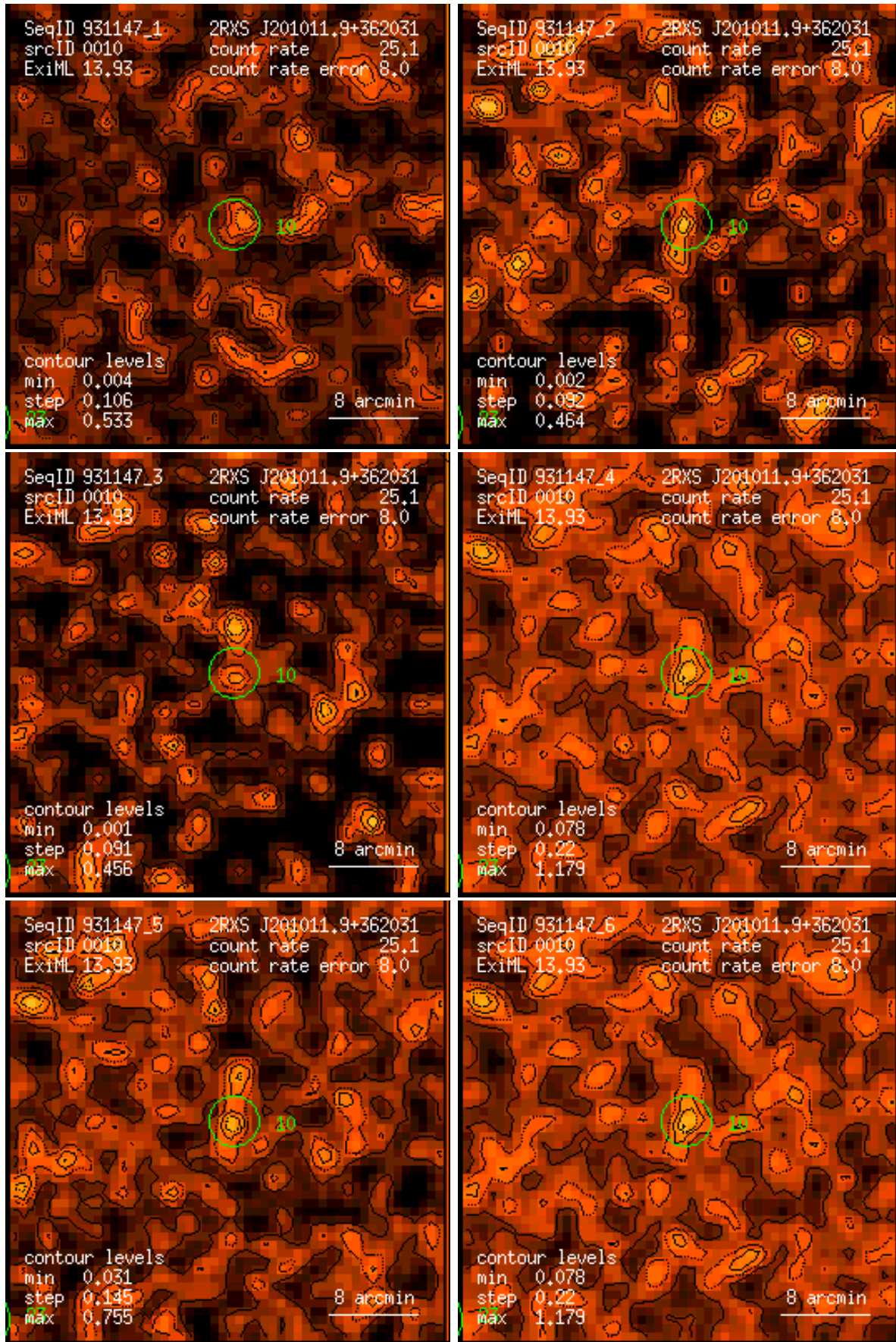
Figure 10: RASS 931147: detection 0010: band rate images, Gaussian filter: (1) PSPC channels 11 – 41, (2) 52 – 90, (3) 91 – 201, (4) 11 – 235, (5) 52 – 201, (6) 11 – 201. Broad band rates in counts/ks. Band rate contour levels in counts/ks/arcmin 2 .
