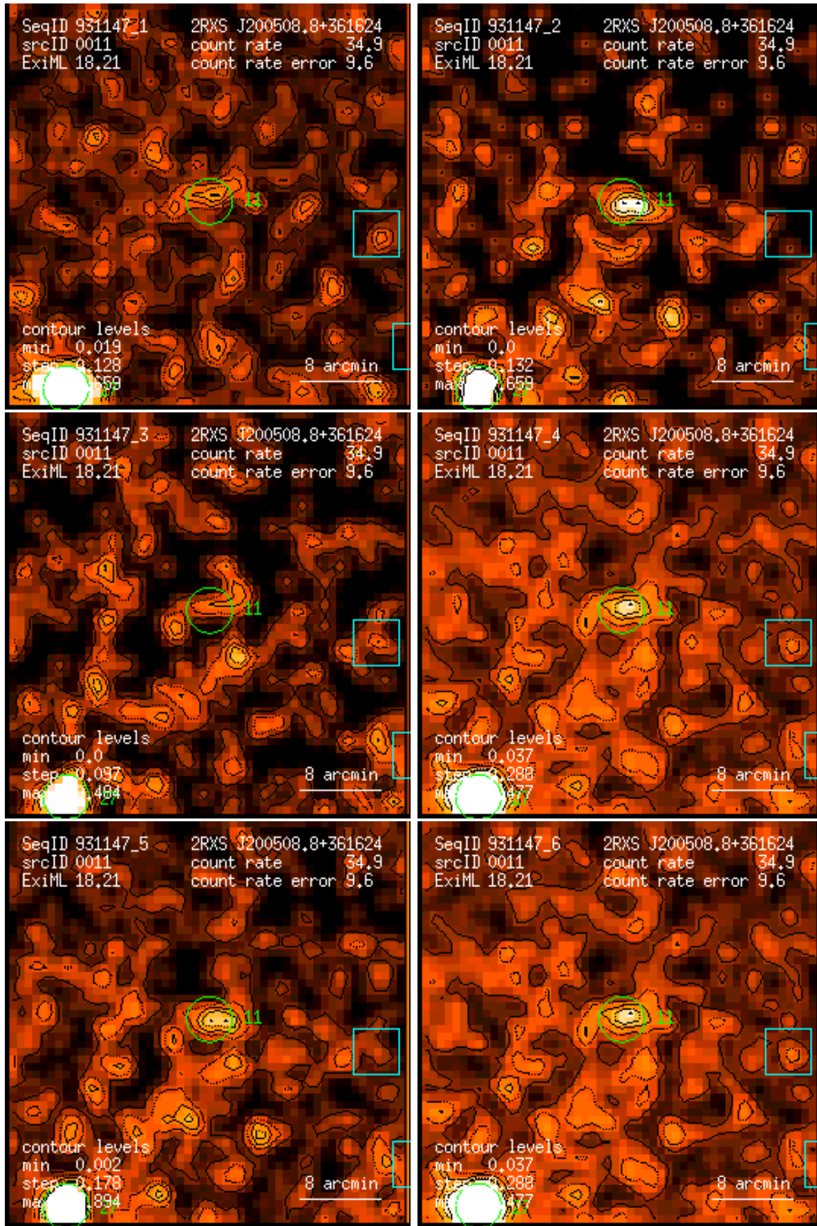
Figure 11: RASS 931147: detection 0011: band rate images, Gaussian filter: (1) PSPC channels 11 – 41, (2) 52 – 90, (3) 91 – 201, (4) 11 – 235, (5) 52 – 201, (6) 11 – 201. Broad band rates in counts/ks. Band rate contour levels in counts/ks/arcmin 2 .
