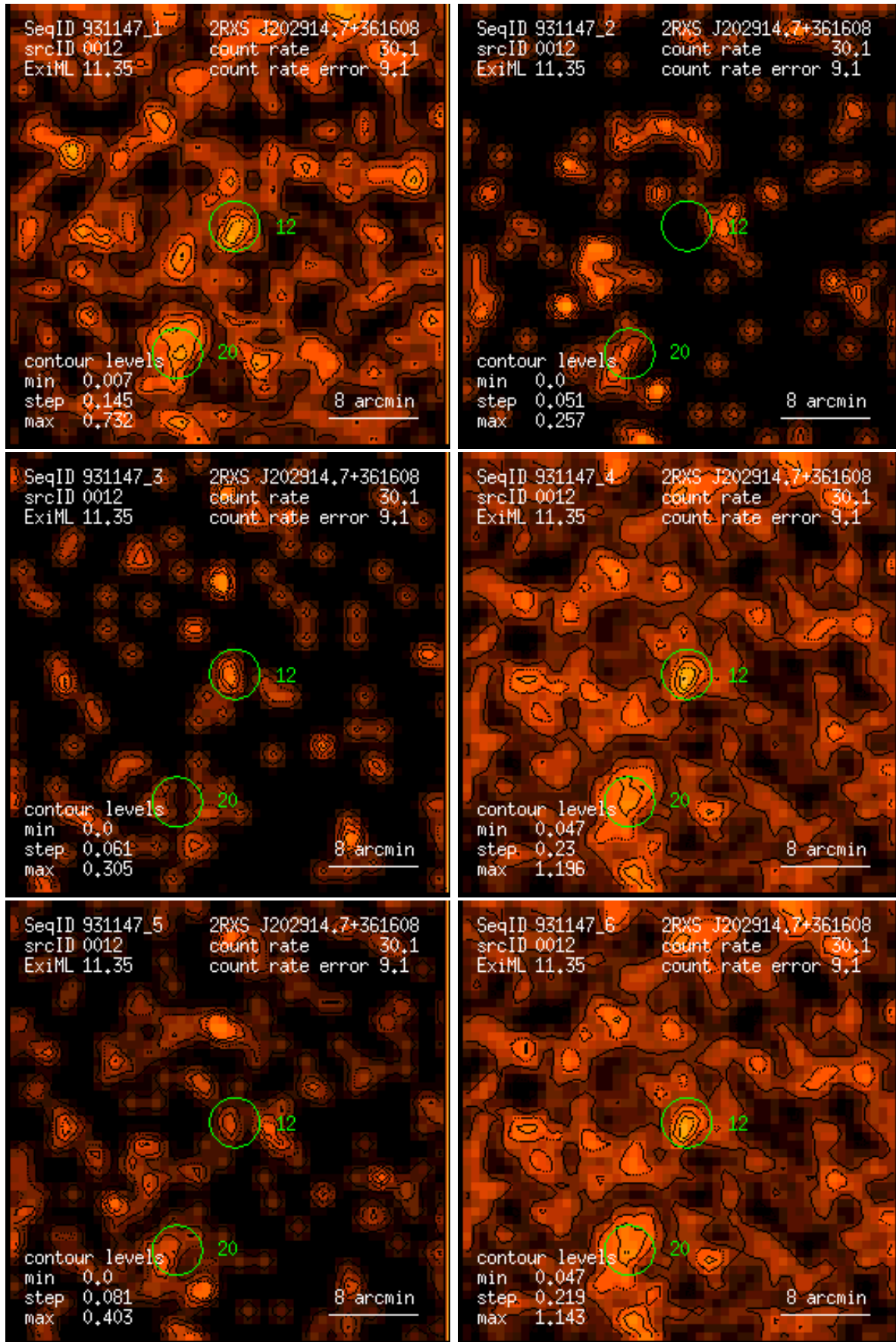
Figure 12: RASS 931147: detection 0012: band rate images, Gaussian filter: (1) PSPC channels 11 – 41, (2) 52 – 90, (3) 91 – 201, (4) 11 – 235, (5) 52 – 201, (6) 11 – 201. Broad band rates in counts/ks. Band rate contour levels in counts/ks/arcmin 2 .
