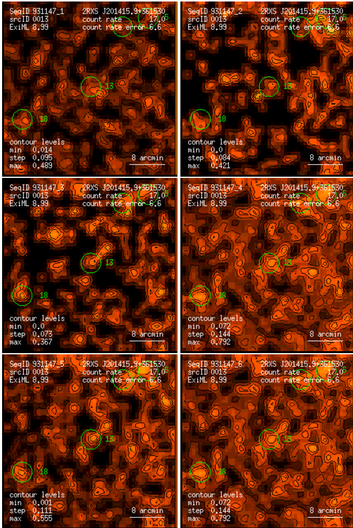
Figure 13: RASS 931147: detection 0013: band rate images, Gaussian filter: (1) PSPC channels 11 – 41, (2) 52 – 90, (3) 91 – 201, (4) 11 – 235, (5) 52 – 201, (6) 11 – 201. Broad band rates in counts/ks. Band rate contour levels in counts/ks/arcmin 2 .
