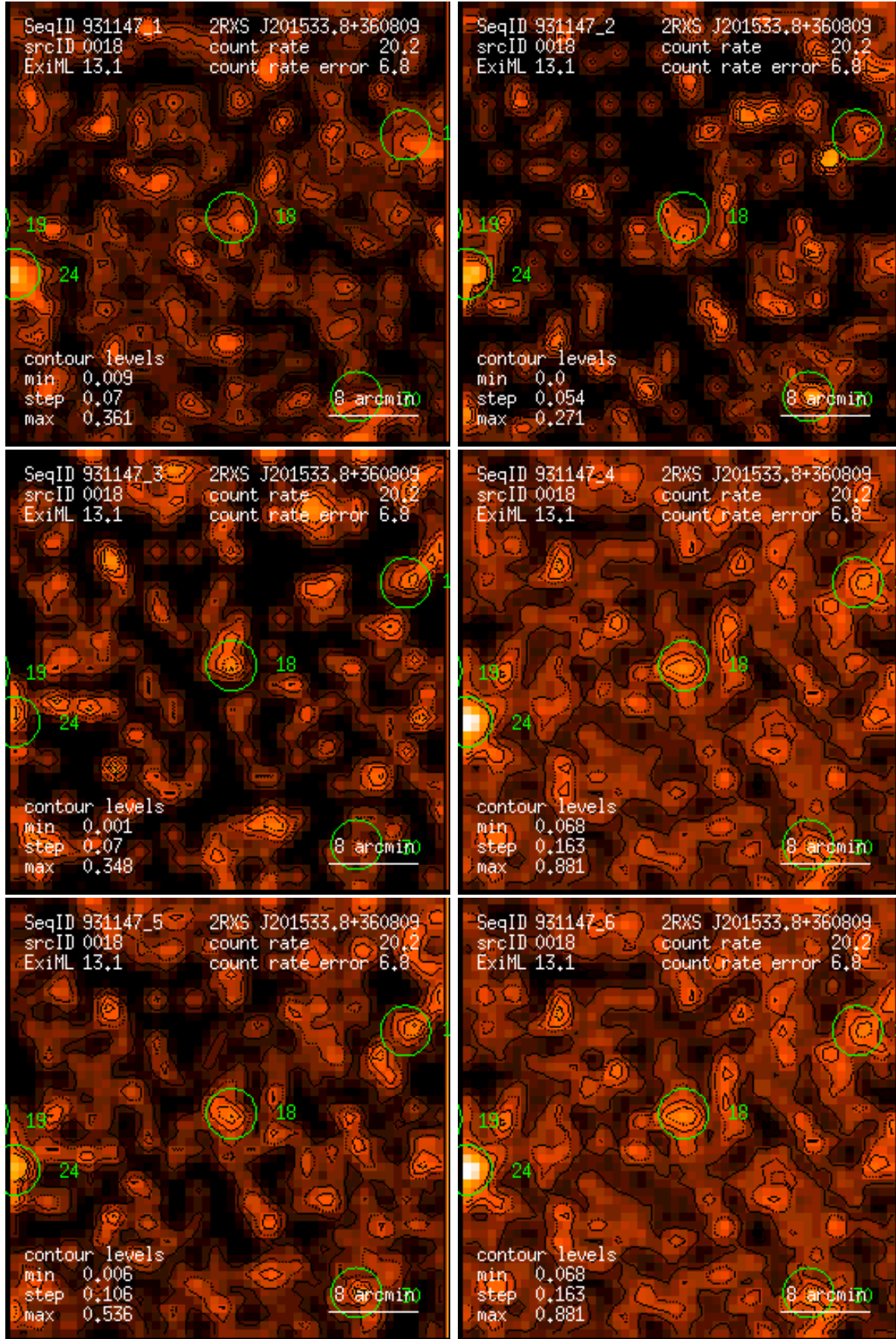
Figure 18: RASS 931147: detection 0018: band rate images, Gaussian filter: (1) PSPC channels 11 – 41, (2) 52 – 90, (3) 91 – 201, (4) 11 – 235, (5) 52 – 201, (6) 11 – 201. Broad band rates in counts/ks. Band rate contour levels in counts/ks/arcmin 2 .
