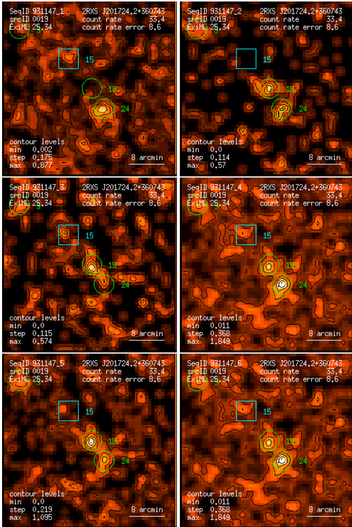
Figure 19: RASS 931147: detection 0019: band rate images, Gaussian filter: (1) PSPC channels 11 – 41, (2) 52 – 90, (3) 91 – 201, (4) 11 – 235, (5) 52 – 201, (6) 11 – 201. Broad band rates in counts/ks. Band rate contour levels in counts/ks/arcmin 2 .
