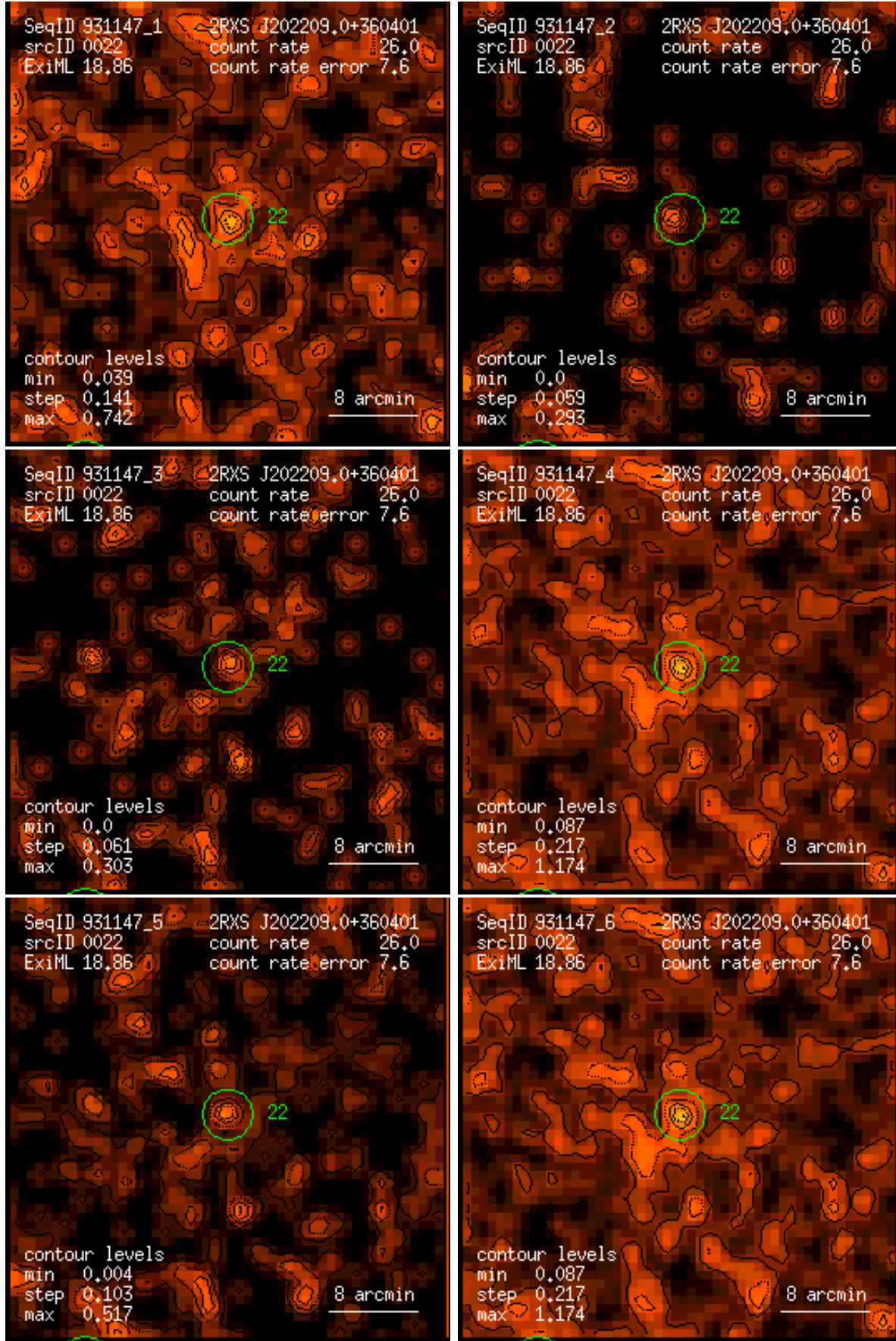
Figure 22: RASS 931147: detection 0022: band rate images, Gaussian filter: (1) PSPC channels 11 – 41, (2) 52 – 90, (3) 91 – 201, (4) 11 – 235, (5) 52 – 201, (6) 11 – 201. Broad band rates in counts/ks. Band rate contour levels in counts/ks/arcmin 2 .
