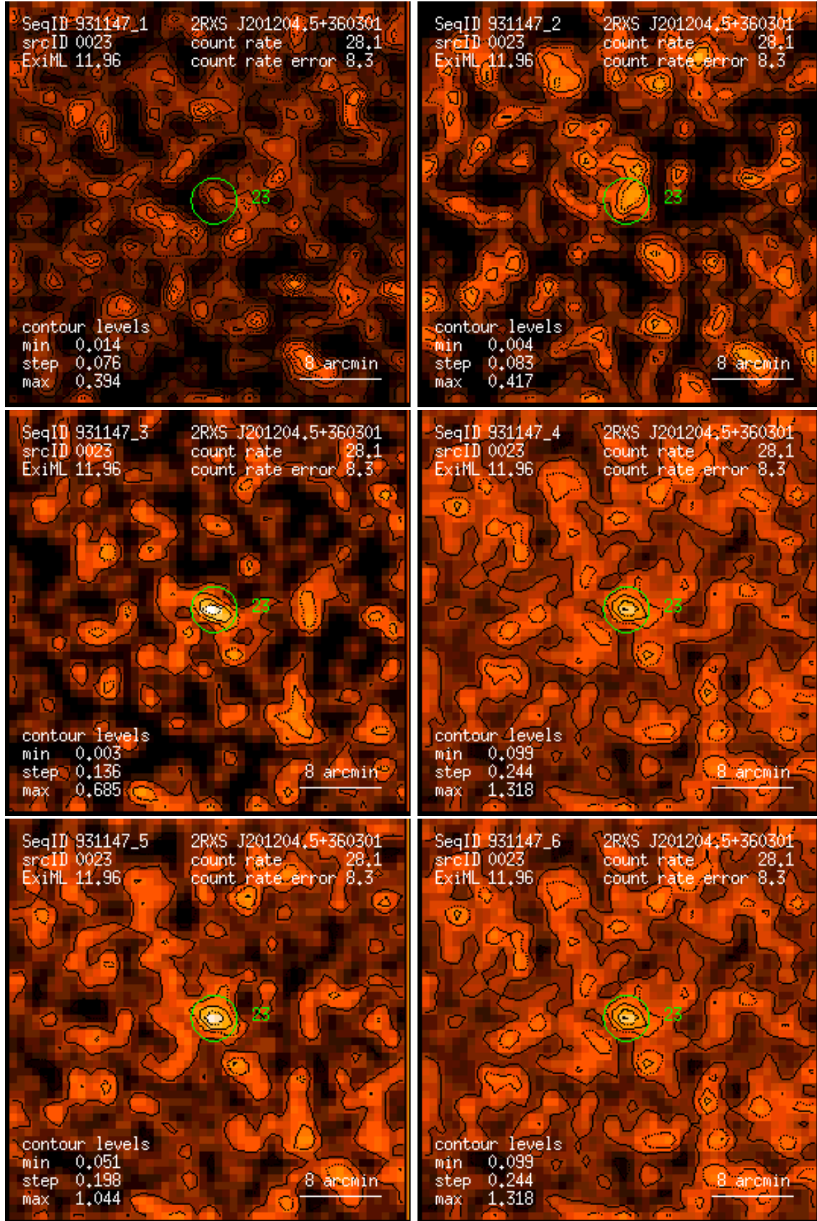
Figure 23: RASS 931147: detection 0023: band rate images, Gaussian filter: (1) PSPC channels 11 – 41, (2) 52 – 90, (3) 91 – 201, (4) 11 – 235, (5) 52 – 201, (6) 11 – 201. Broad band rates in counts/ks. Band rate contour levels in counts/ks/arcmin 2 .
