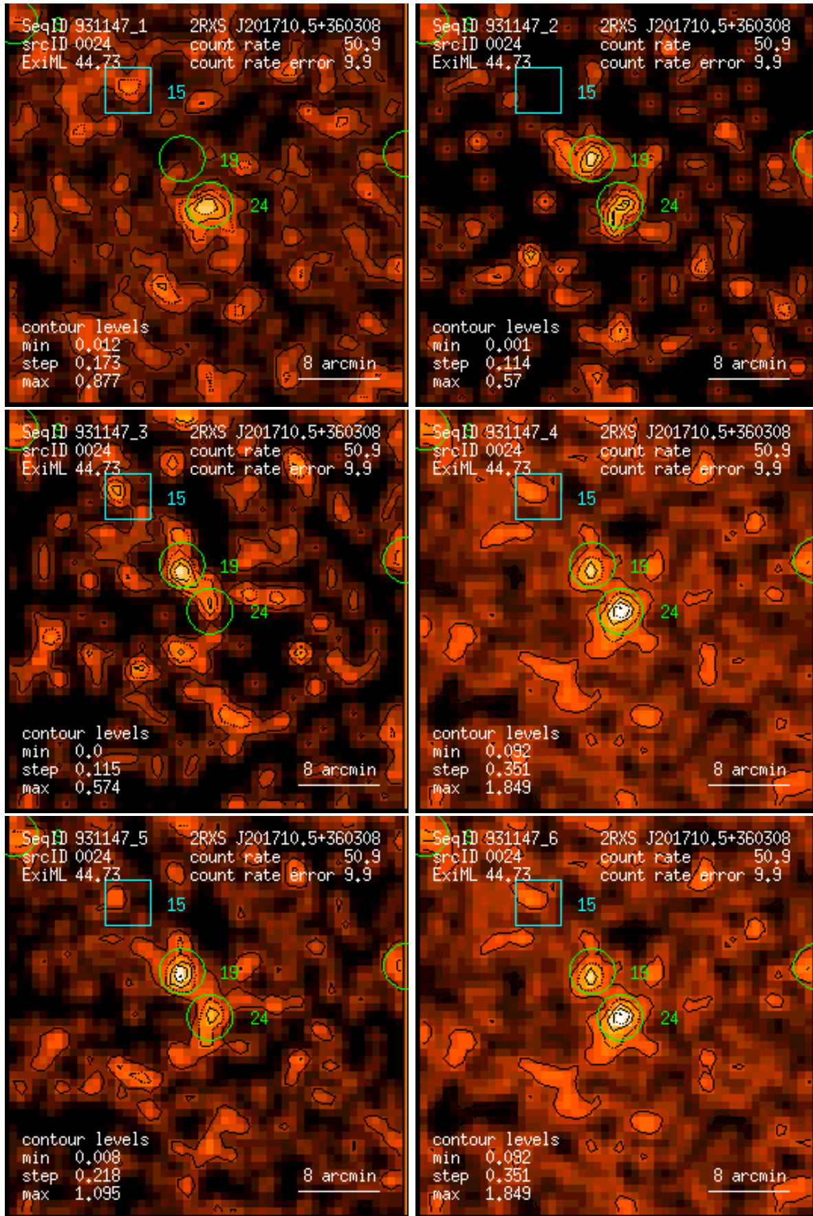
Figure 24: RASS 931147: detection 0024: band rate images, Gaussian filter: (1) PSPC channels 11 – 41, (2) 52 – 90, (3) 91 – 201, (4) 11 – 235, (5) 52 – 201, (6) 11 – 201. Broad band rates in counts/ks. Band rate contour levels in counts/ks/arcmin 2 .
