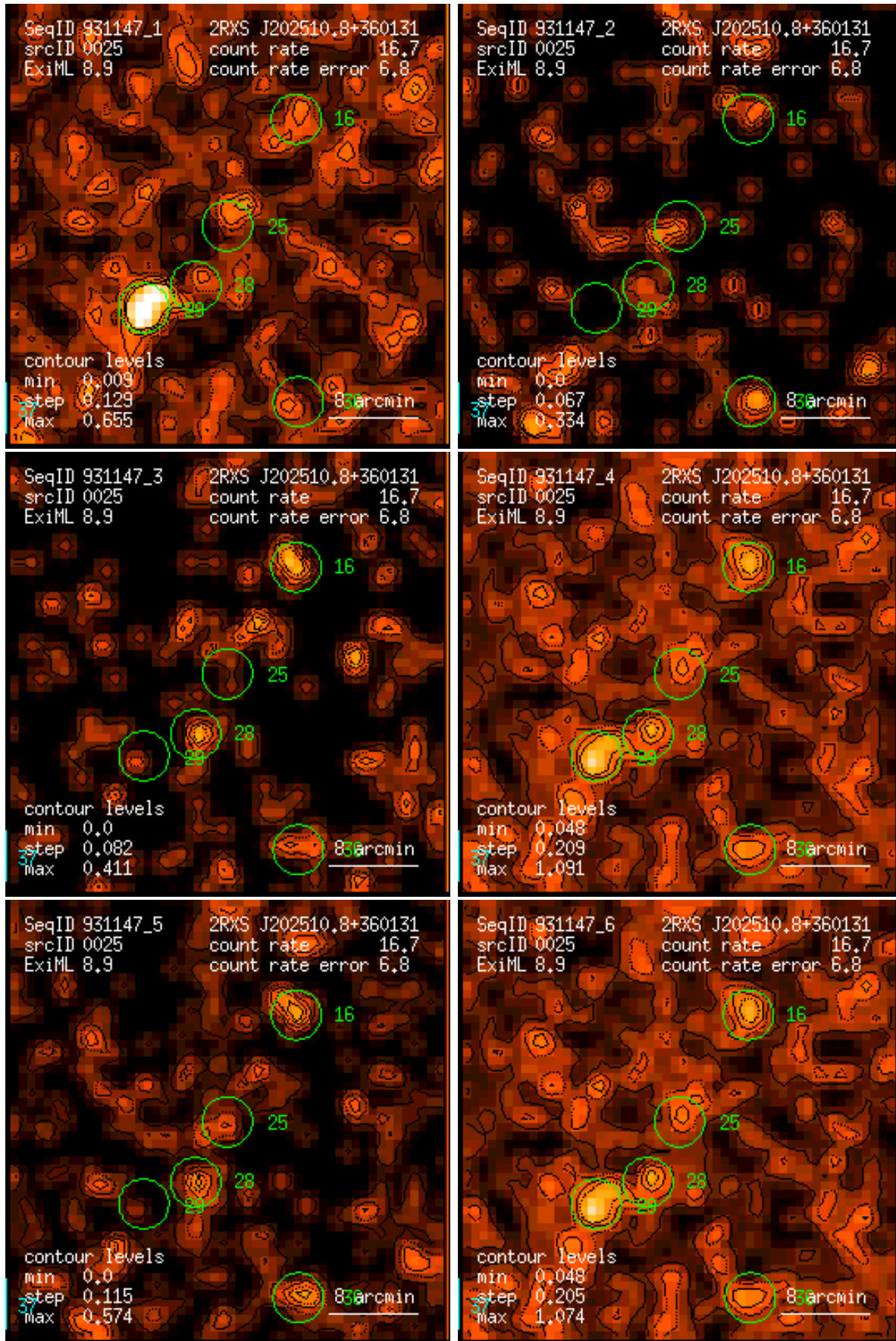
Figure 25: RASS 931147: detection 0025: band rate images, Gaussian filter: (1) PSPC channels 11 – 41, (2) 52 – 90, (3) 91 – 201, (4) 11 – 235, (5) 52 – 201, (6) 11 – 201. Broad band rates in counts/ks. Band rate contour levels in counts/ks/arcmin 2 .
