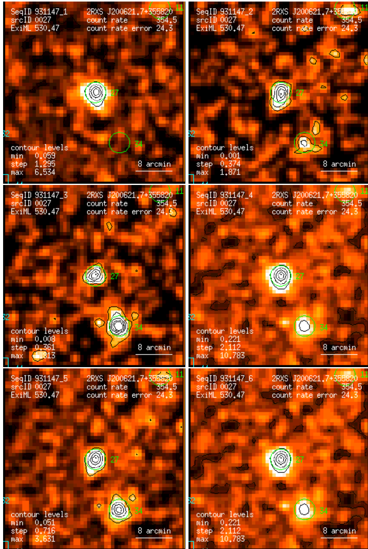
Figure 27: RASS 931147: detection 0027: band rate images, Gaussian filter: (1) PSPC channels 11 – 41, (2) 52 – 90, (3) 91 – 201, (4) 11 – 235, (5) 52 – 201, (6) 11 – 201. Broad band rates in counts/ks. Band rate contour levels in counts/ks/arcmin 2 .
