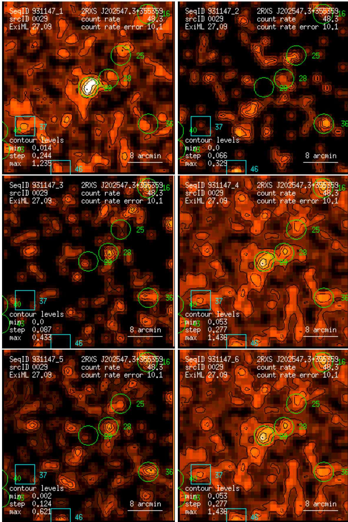
Figure 29: RASS 931147: detection 0029: band rate images, Gaussian filter: (1) PSPC channels 11 – 41, (2) 52 – 90, (3) 91 – 201, (4) 11 – 235, (5) 52 – 201, (6) 11 – 201. Broad band rates in counts/ks. Band rate contour levels in counts/ks/arcmin 2 .
