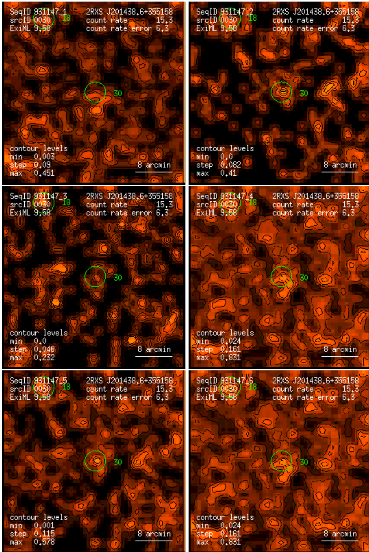
Figure 30: RASS 931147: detection 0030: band rate images, Gaussian filter: (1) PSPC channels 11 – 41, (2) 52 – 90, (3) 91 – 201, (4) 11 – 235, (5) 52 – 201, (6) 11 – 201. Broad band rates in counts/ks. Band rate contour levels in counts/ks/arcmin 2 .
