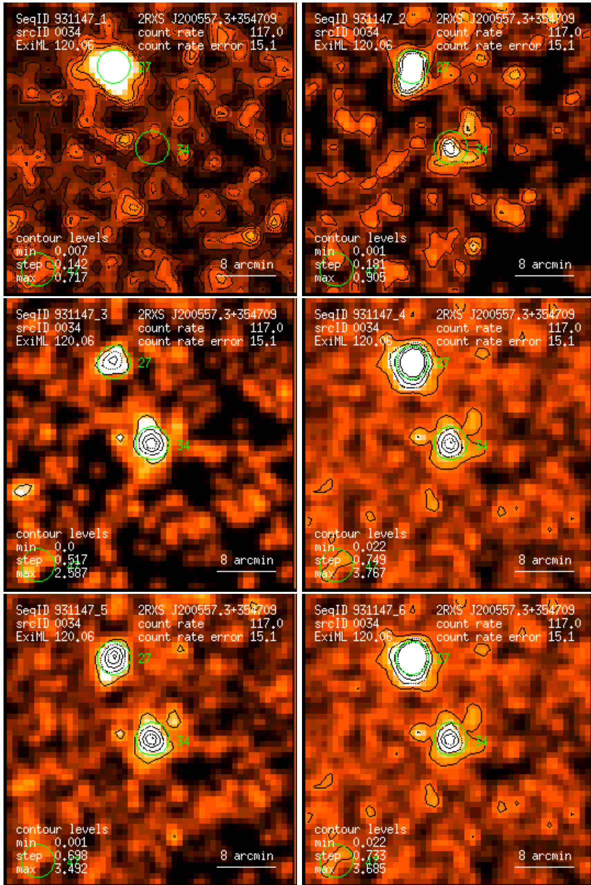
Figure 34: RASS 931147: detection 0034: band rate images, Gaussian filter: (1) PSPC channels 11 – 41, (2) 52 – 90, (3) 91 – 201, (4) 11 – 235, (5) 52 – 201, (6) 11 – 201. Broad band rates in counts/ks. Band rate contour levels in counts/ks/arcmin 2 .
