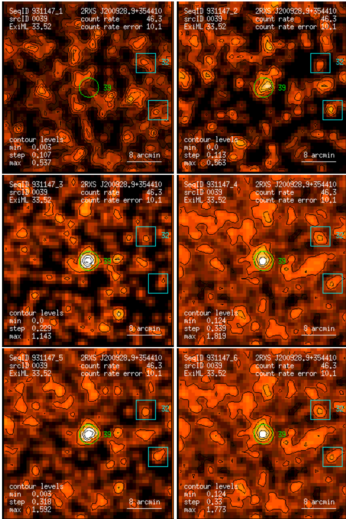
Figure 39: RASS 931147: detection 0039: band rate images, Gaussian filter: (1) PSPC channels 11 – 41, (2) 52 – 90, (3) 91 – 201, (4) 11 – 235, (5) 52 – 201, (6) 11 – 201. Broad band rates in counts/ks. Band rate contour levels in counts/ks/arcmin 2 .
