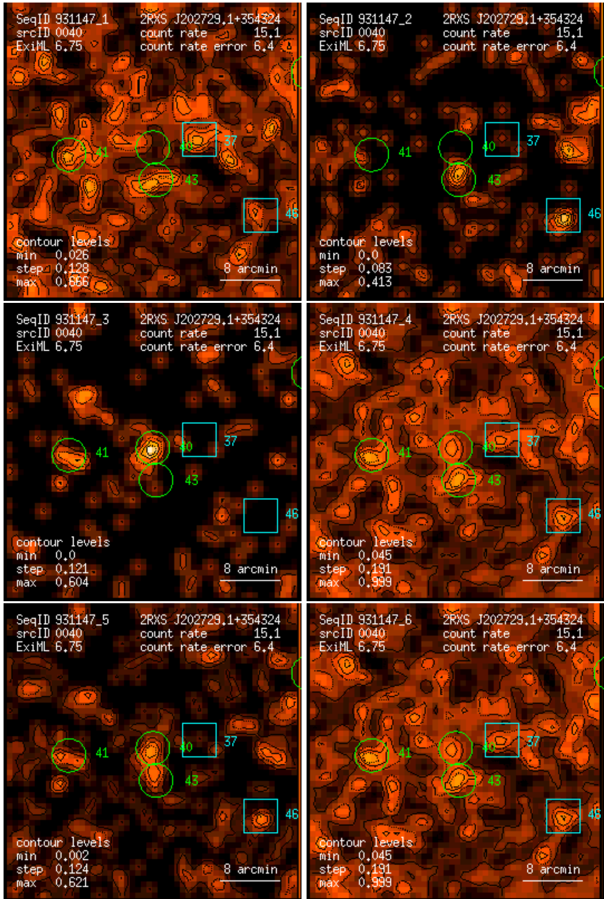
Figure 40: RASS 931147: detection 0040: band rate images, Gaussian filter: (1) PSPC channels 11 – 41, (2) 52 – 90, (3) 91 – 201, (4) 11 – 235, (5) 52 – 201, (6) 11 – 201. Broad band rates in counts/ks. Band rate contour levels in counts/ks/arcmin 2 .
