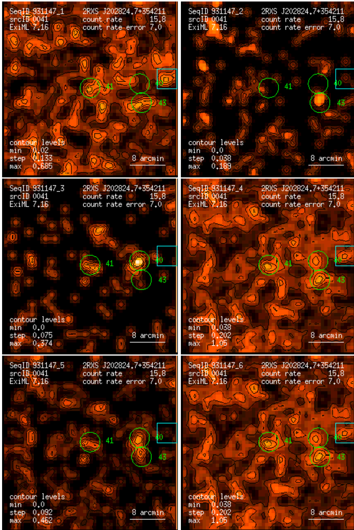
Figure 41: RASS 931147: detection 0041: band rate images, Gaussian filter: (1) PSPC channels 11 – 41, (2) 52 – 90, (3) 91 – 201, (4) 11 – 235, (5) 52 – 201, (6) 11 – 201. Broad band rates in counts/ks. Band rate contour levels in counts/ks/arcmin 2 .
