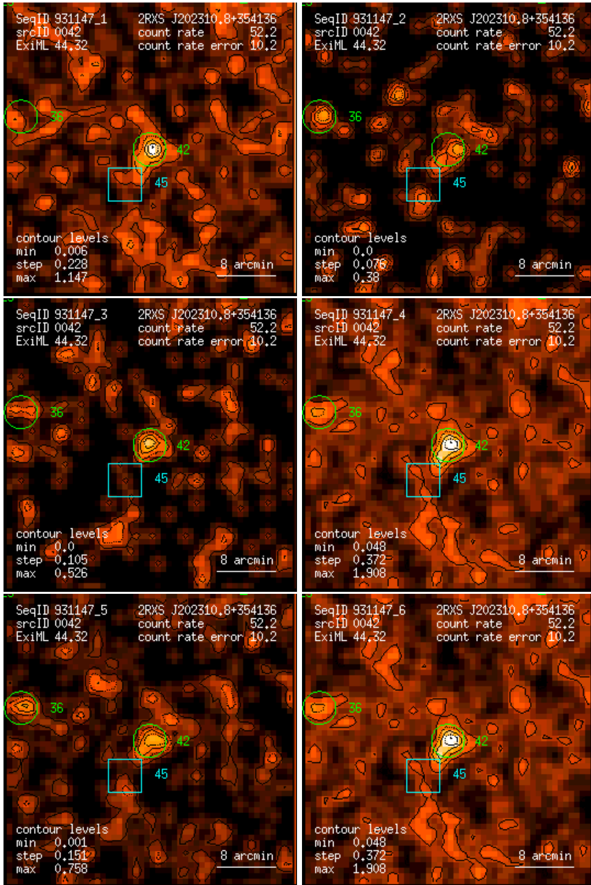
Figure 42: RASS 931147: detection 0042: band rate images, Gaussian filter: (1) PSPC channels 11 – 41, (2) 52 – 90, (3) 91 – 201, (4) 11 – 235, (5) 52 – 201, (6) 11 – 201. Broad band rates in counts/ks. Band rate contour levels in counts/ks/arcmin 2 .
