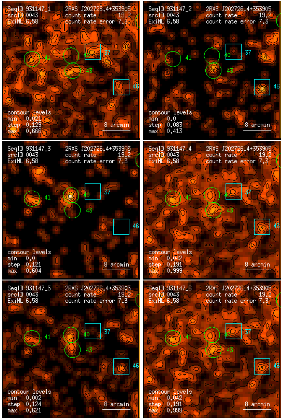
Figure 43: RASS 931147: detection 0043: band rate images, Gaussian filter: (1) PSPC channels 11 – 41, (2) 52 – 90, (3) 91 – 201, (4) 11 – 235, (5) 52 – 201, (6) 11 – 201. Broad band rates in counts/ks. Band rate contour levels in counts/ks/arcmin 2 .
