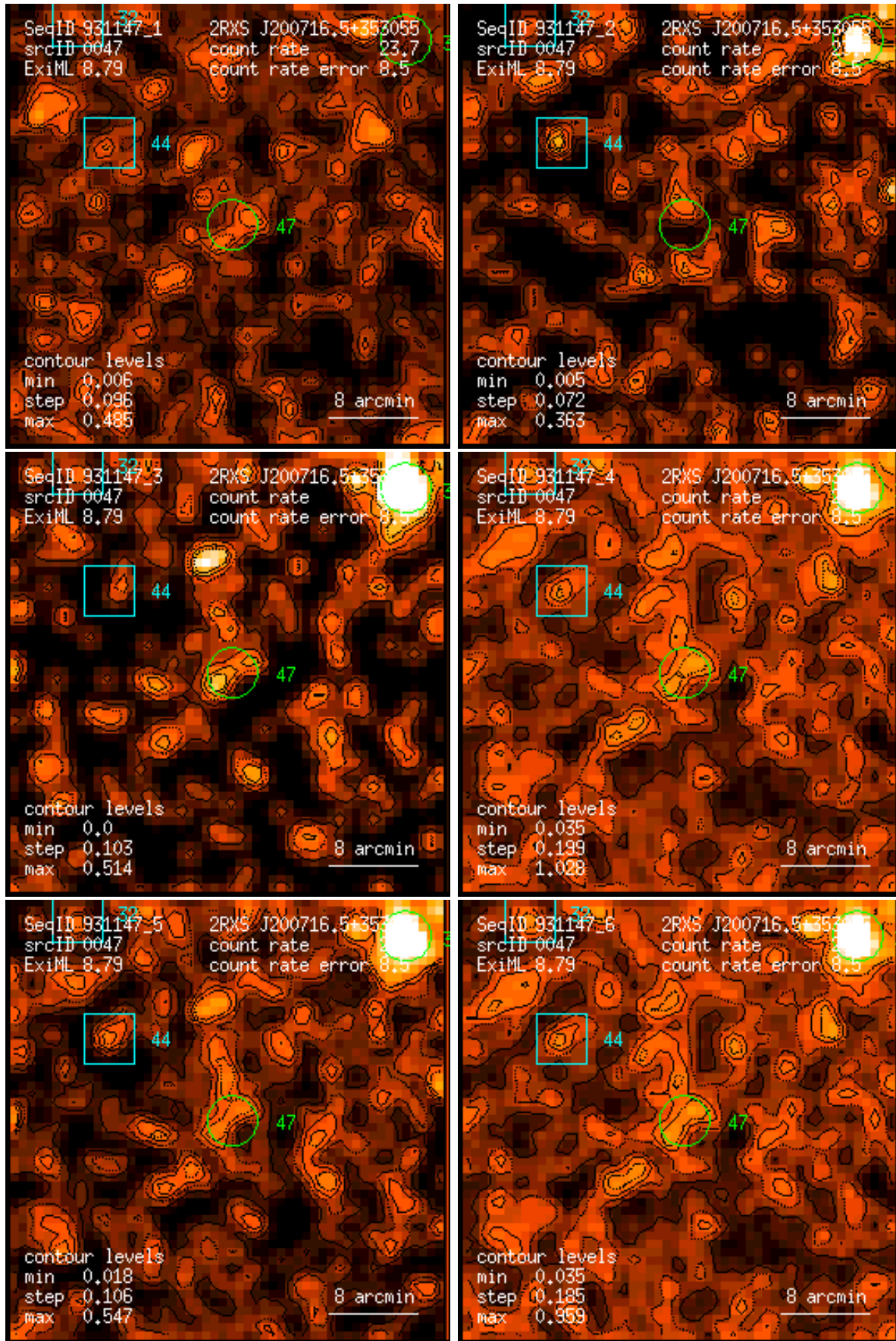
Figure 47: RASS 931147: detection 0047: band rate images, Gaussian filter: (1) PSPC channels 11 – 41, (2) 52 – 90, (3) 91 – 201, (4) 11 – 235, (5) 52 – 201, (6) 11 – 201. Broad band rates in counts/ks. Band rate contour levels in counts/ks/arcmin 2 .
