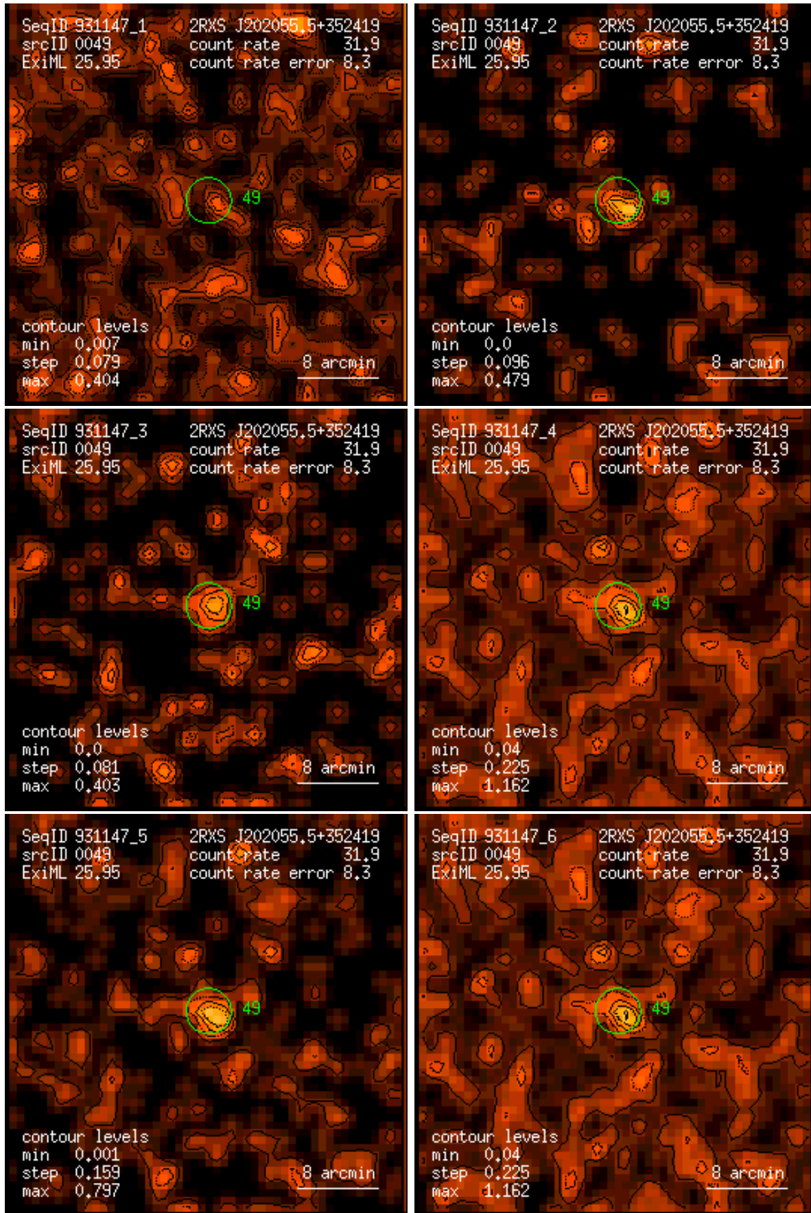
Figure 49: RASS 931147: detection 0049: band rate images, Gaussian filter: (1) PSPC channels 11 – 41, (2) 52 – 90, (3) 91 – 201, (4) 11 – 235, (5) 52 – 201, (6) 11 – 201. Broad band rates in counts/ks. Band rate contour levels in counts/ks/arcmin 2 .
