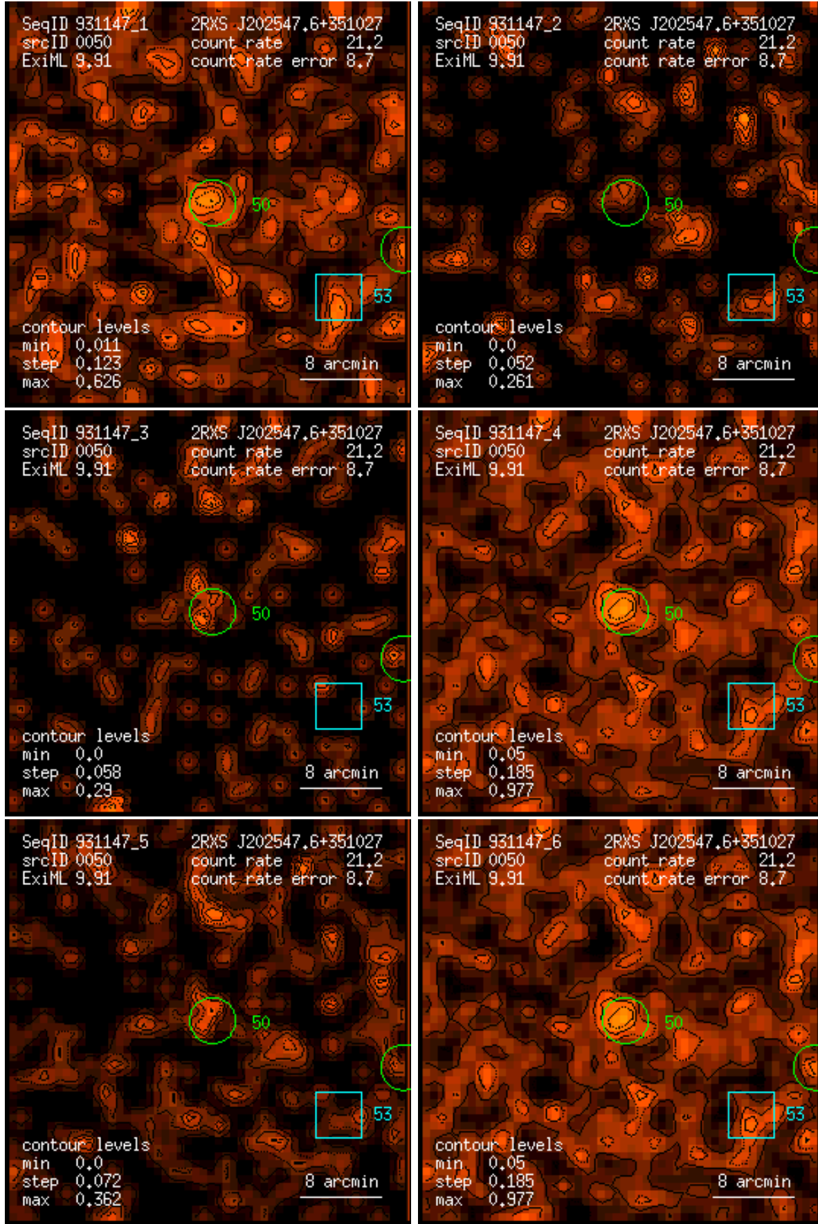
Figure 50: RASS 931147: detection 0050: band rate images, Gaussian filter: (1) PSPC channels 11 – 41, (2) 52 – 90, (3) 91 – 201, (4) 11 – 235, (5) 52 – 201, (6) 11 – 201. Broad band rates in counts/ks. Band rate contour levels in counts/ks/arcmin 2 .
