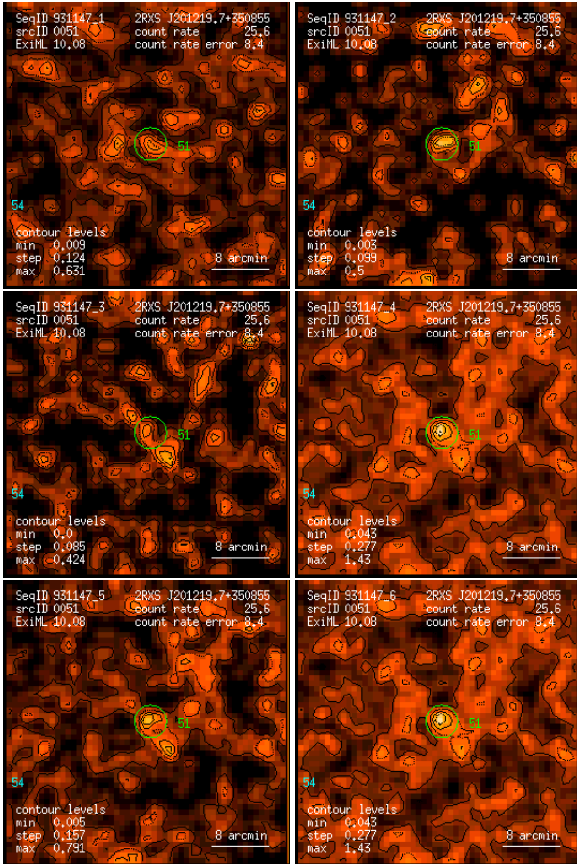
Figure 51: RASS 931147: detection 0051: band rate images, Gaussian filter: (1) PSPC channels 11 – 41, (2) 52 – 90, (3) 91 – 201, (4) 11 – 235, (5) 52 – 201, (6) 11 – 201. Broad band rates in counts/ks. Band rate contour levels in counts/ks/arcmin 2 .
