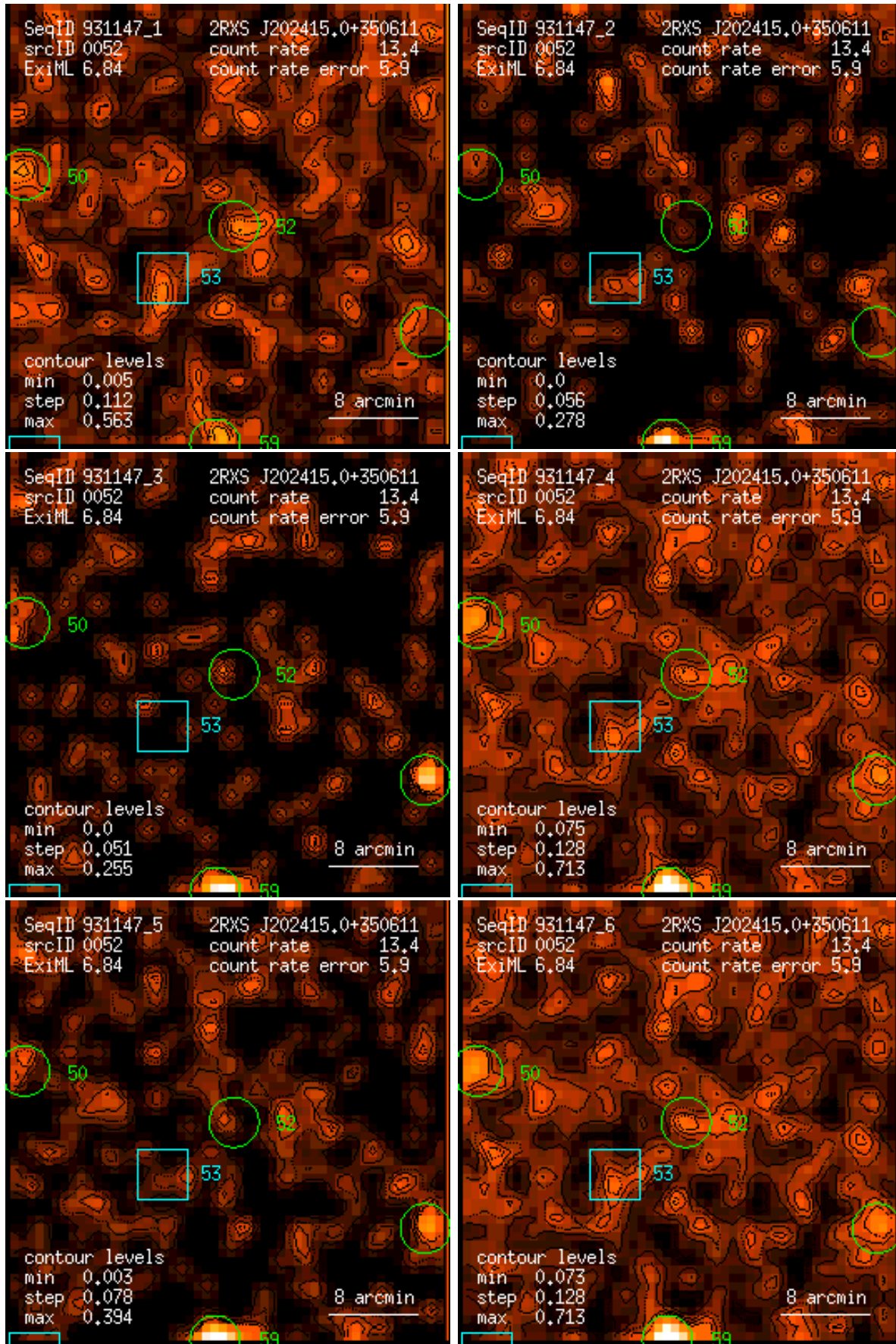
Figure 52: RASS 931147: detection 0052: band rate images, Gaussian filter: (1) PSPC channels 11 – 41, (2) 52 – 90, (3) 91 – 201, (4) 11 – 235, (5) 52 – 201, (6) 11 – 201. Broad band rates in counts/ks. Band rate contour levels in counts/ks/arcmin 2 .
