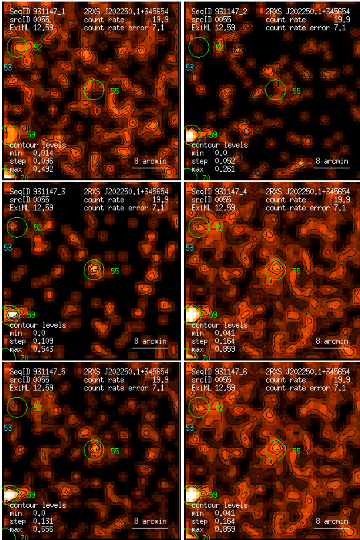
Figure 55: RASS 931147: detection 0055: band rate images, Gaussian filter: (1) PSPC channels 11 – 41, (2) 52 – 90, (3) 91 – 201, (4) 11 – 235, (5) 52 – 201, (6) 11 – 201. Broad band rates in counts/ks. Band rate contour levels in counts/ks/arcmin 2 .
