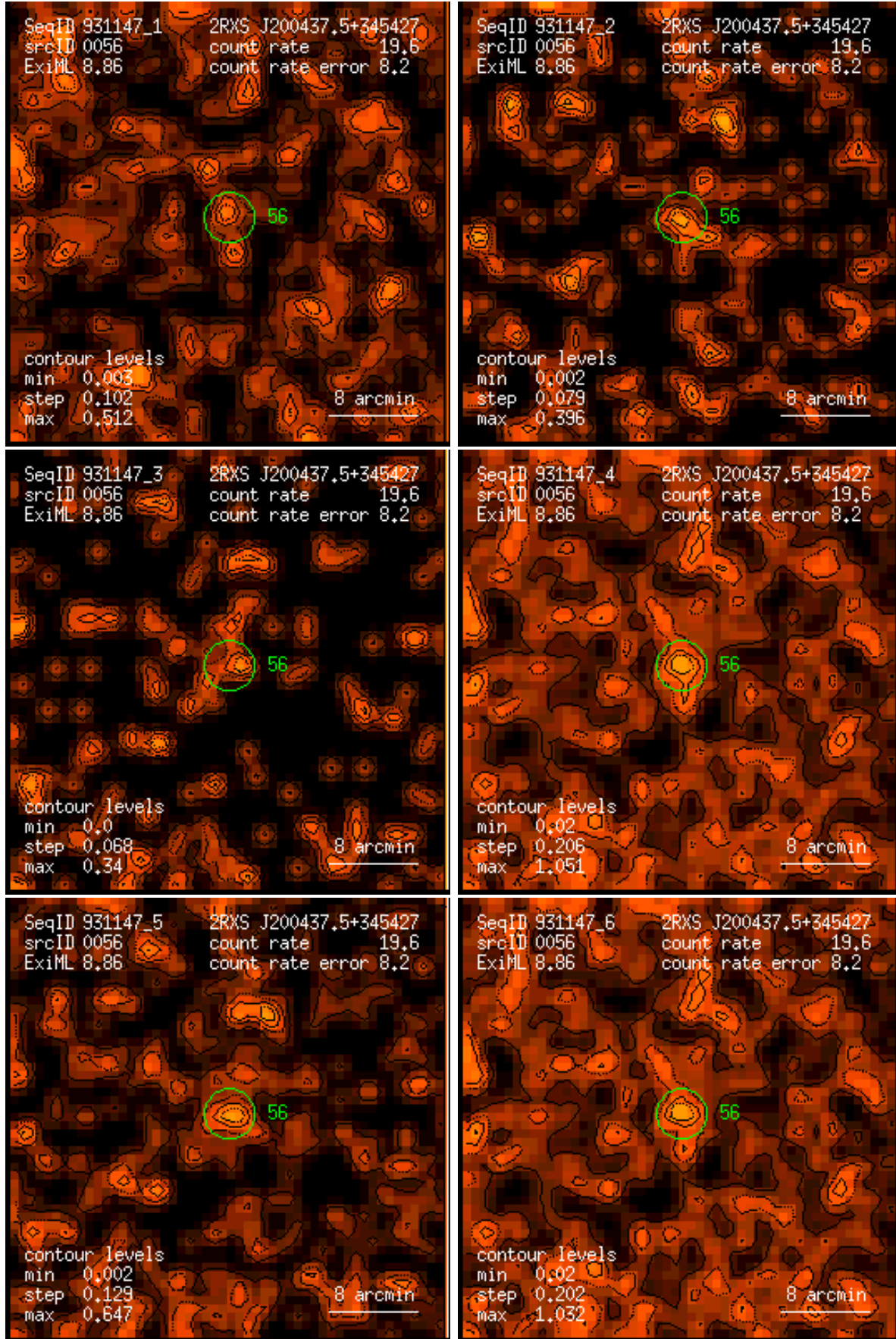
Figure 56: RASS 931147: detection 0056: band rate images, Gaussian filter: (1) PSPC channels 11 – 41, (2) 52 – 90, (3) 91 – 201, (4) 11 – 235, (5) 52 – 201, (6) 11 – 201. Broad band rates in counts/ks. Band rate contour levels in counts/ks/arcmin 2 .
