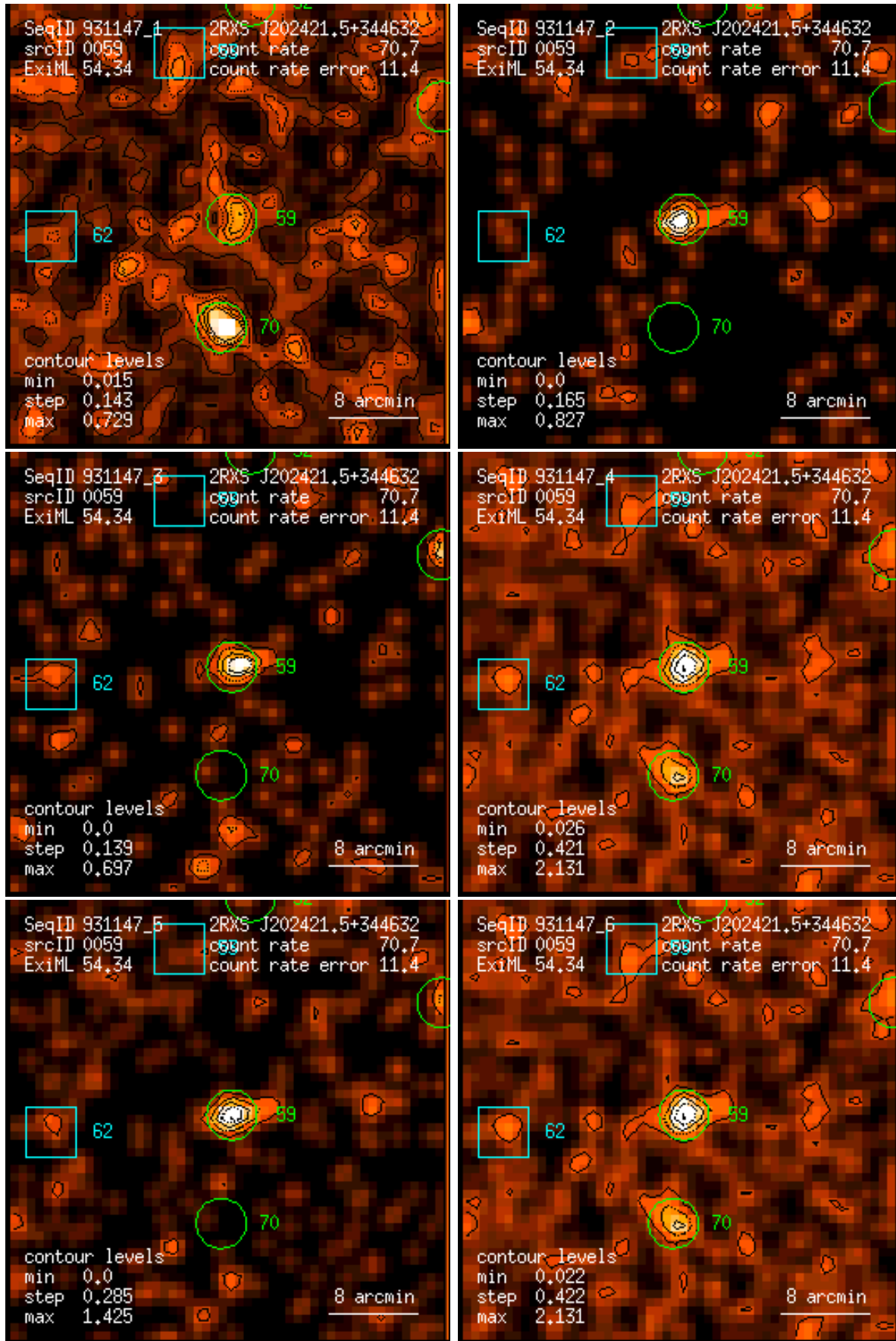
Figure 59: RASS 931147: detection 0059: band rate images, Gaussian filter: (1) PSPC channels 11 – 41, (2) 52 – 90, (3) 91 – 201, (4) 11 – 235, (5) 52 – 201, (6) 11 – 201. Broad band rates in counts/ks. Band rate contour levels in counts/ks/arcmin 2 .
