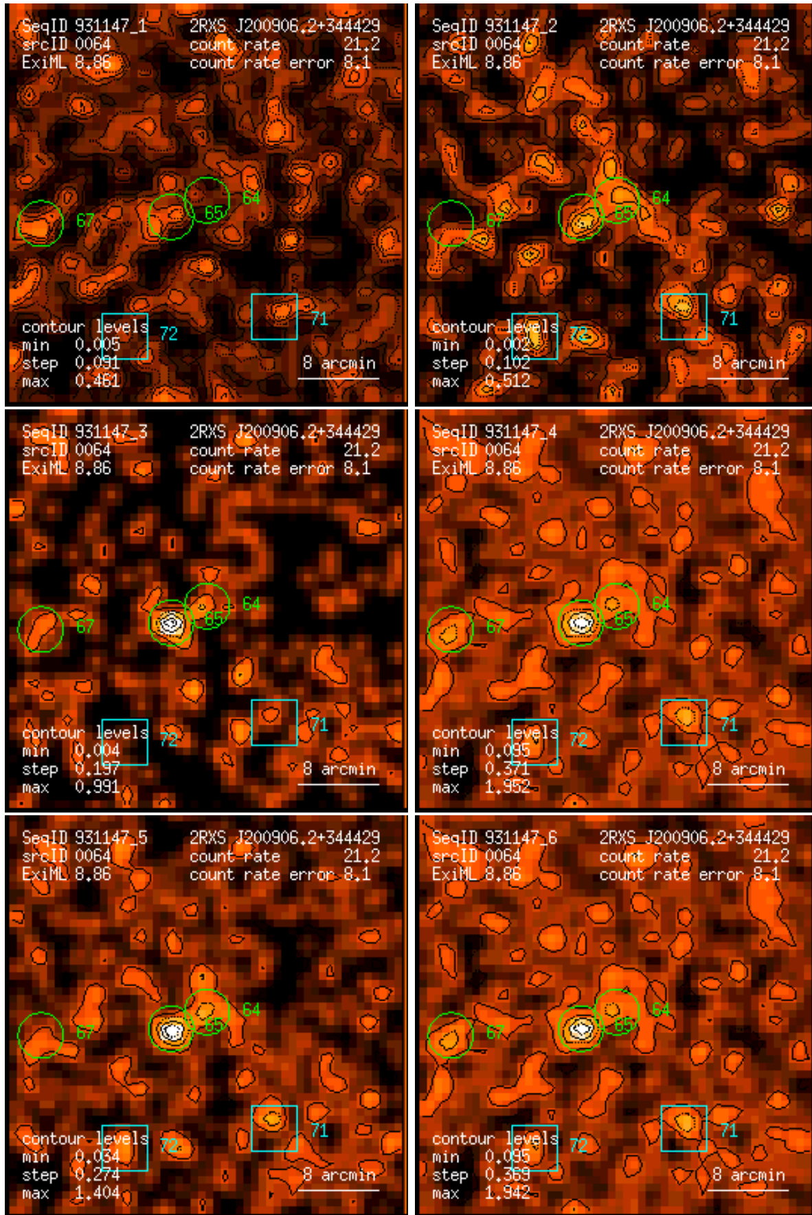
Figure 64: RASS 931147: detection 0064: band rate images, Gaussian filter: (1) PSPC channels 11 – 41, (2) 52 – 90, (3) 91 – 201, (4) 11 – 235, (5) 52 – 201, (6) 11 – 201. Broad band rates in counts/ks. Band rate contour levels in counts/ks/arcmin 2 .
