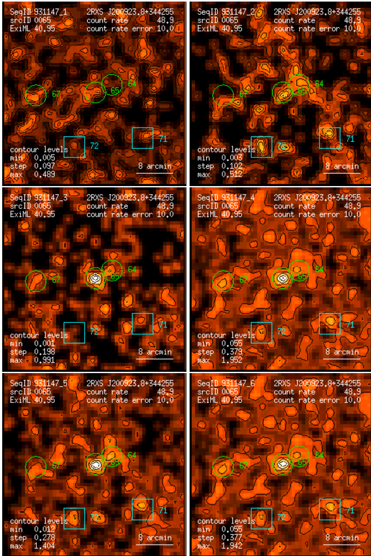
Figure 65: RASS 931147: detection 0065: band rate images, Gaussian filter: (1) PSPC channels 11 – 41, (2) 52 – 90, (3) 91 – 201, (4) 11 – 235, (5) 52 – 201, (6) 11 – 201. Broad band rates in counts/ks. Band rate contour levels in counts/ks/arcmin 2 .
