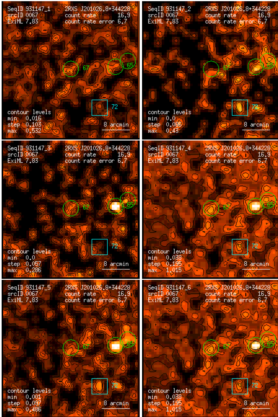
Figure 67: RASS 931147: detection 0067: band rate images, Gaussian filter: (1) PSPC channels 11 – 41, (2) 52 – 90, (3) 91 – 201, (4) 11 – 235, (5) 52 – 201, (6) 11 – 201. Broad band rates in counts/ks. Band rate contour levels in counts/ks/arcmin 2 .
