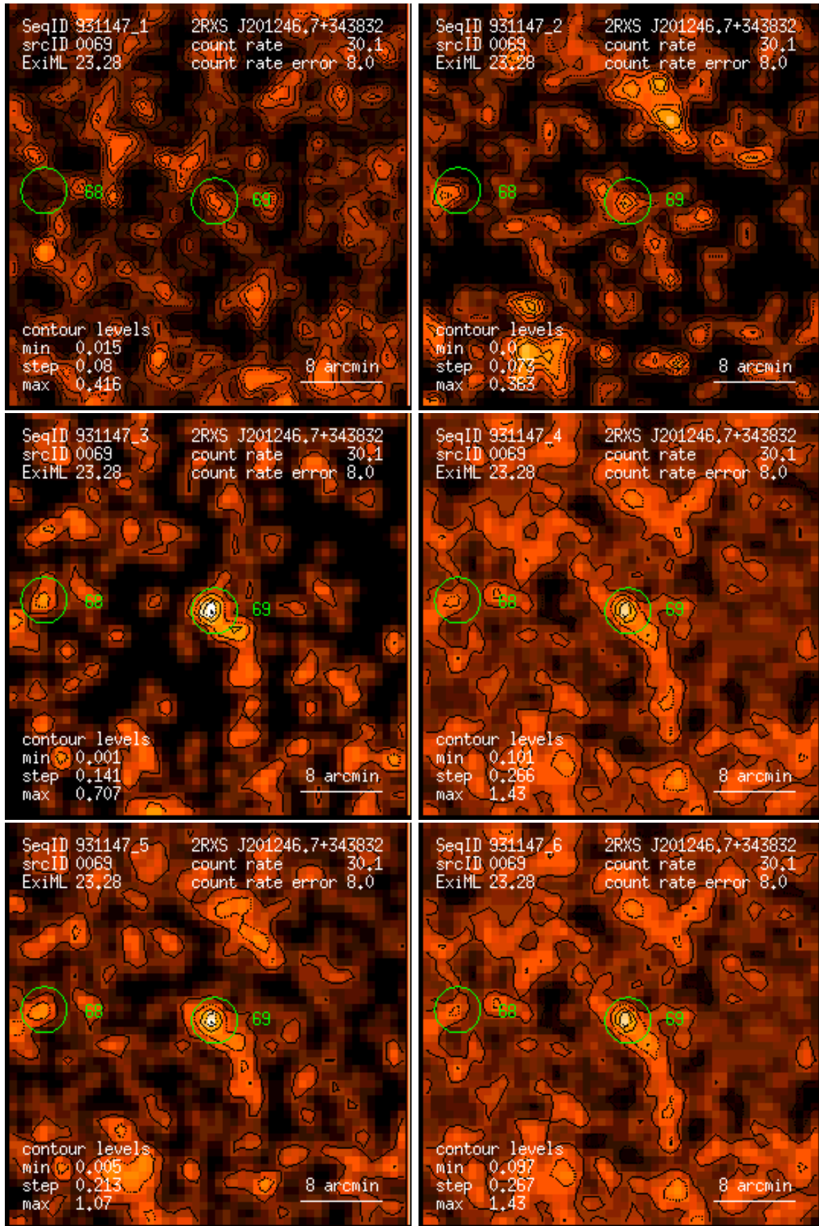
Figure 69: RASS 931147: detection 0069: band rate images, Gaussian filter: (1) PSPC channels 11 – 41, (2) 52 – 90, (3) 91 – 201, (4) 11 – 235, (5) 52 – 201, (6) 11 – 201. Broad band rates in counts/ks. Band rate contour levels in counts/ks/arcmin 2 .
