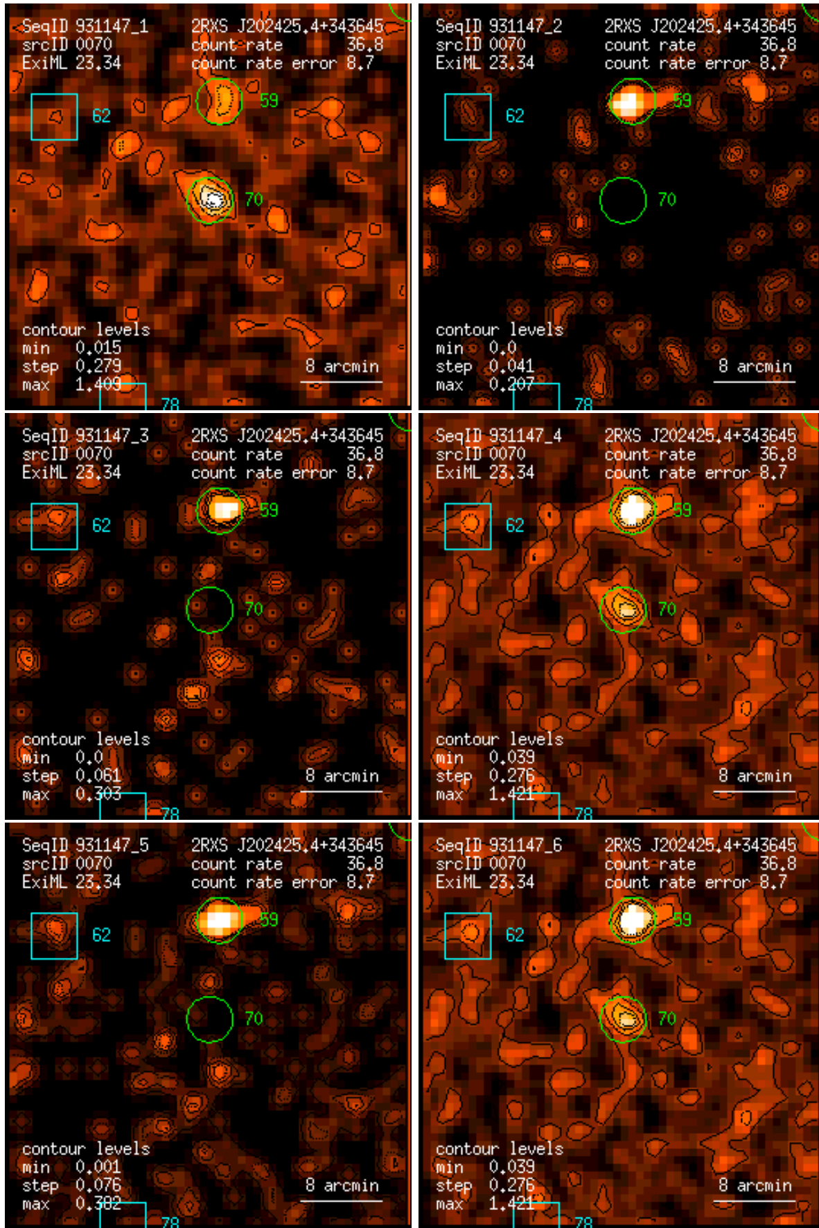
Figure 70: RASS 931147: detection 0070: band rate images, Gaussian filter: (1) PSPC channels 11 – 41, (2) 52 – 90, (3) 91 – 201, (4) 11 – 235, (5) 52 – 201, (6) 11 – 201. Broad band rates in counts/ks. Band rate contour levels in counts/ks/arcmin 2 .
