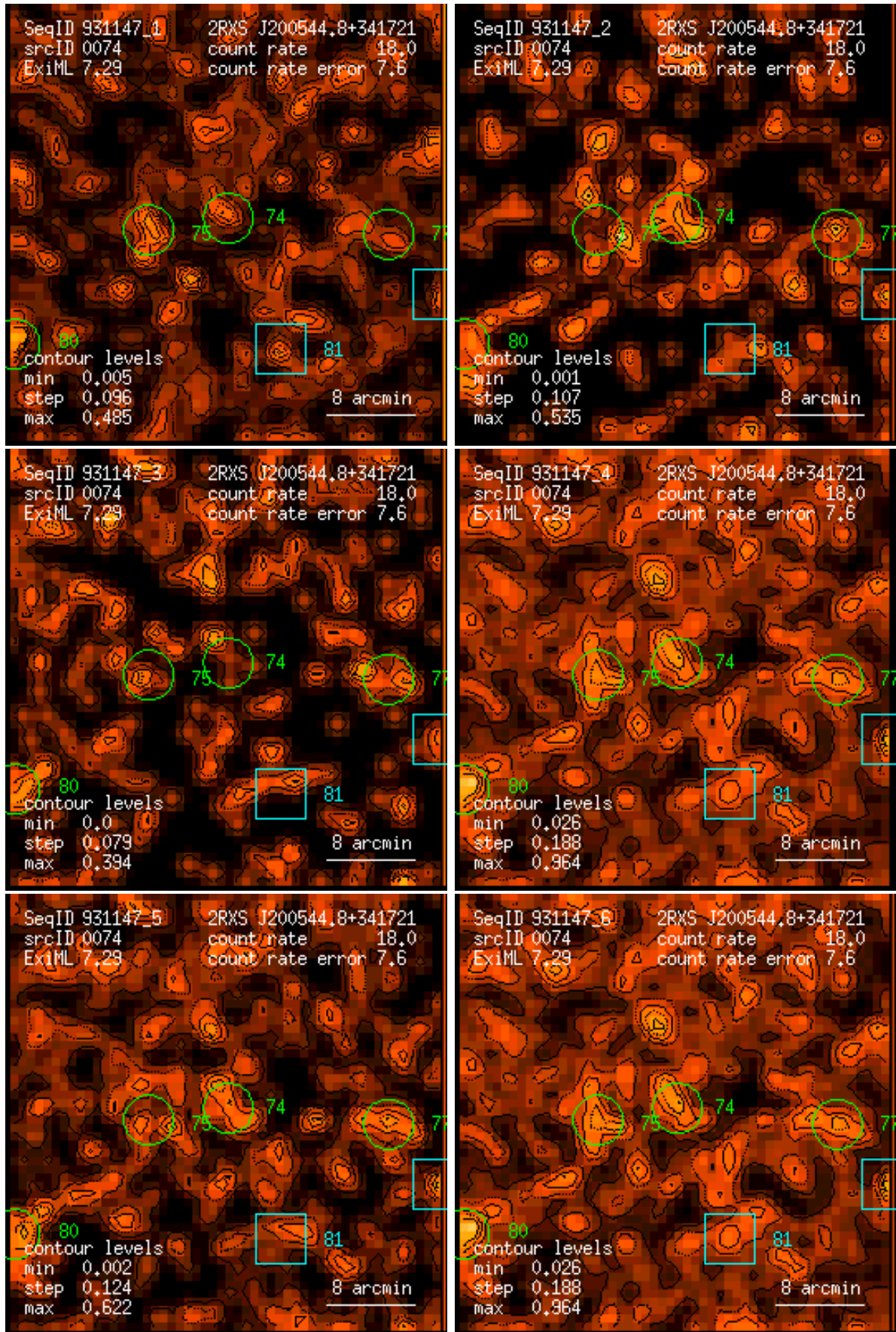
Figure 74: RASS 931147: detection 0074: band rate images, Gaussian filter: (1) PSPC channels 11 – 41, (2) 52 – 90, (3) 91 – 201, (4) 11 – 235, (5) 52 – 201, (6) 11 – 201. Broad band rates in counts/ks. Band rate contour levels in counts/ks/arcmin 2 .
