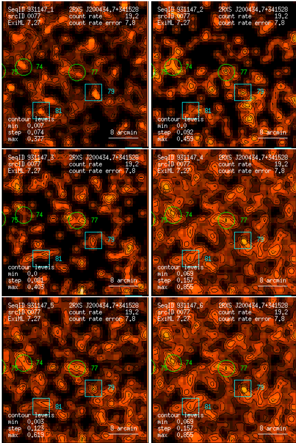
Figure 77: RASS 931147: detection 0077: band rate images, Gaussian filter: (1) PSPC channels 11 – 41, (2) 52 – 90, (3) 91 – 201, (4) 11 – 235, (5) 52 – 201, (6) 11 – 201. Broad band rates in counts/ks. Band rate contour levels in counts/ks/arcmin 2 .
