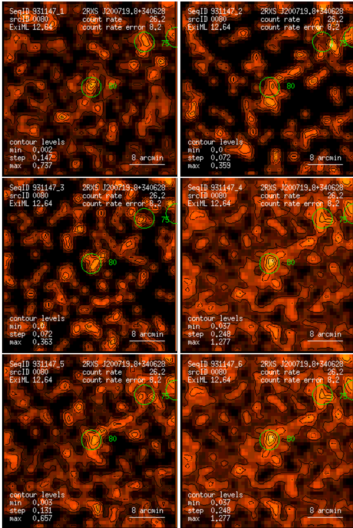
Figure 80: RASS 931147: detection 0080: band rate images, Gaussian filter: (1) PSPC channels 11 – 41, (2) 52 – 90, (3) 91 – 201, (4) 11 – 235, (5) 52 – 201, (6) 11 – 201. Broad band rates in counts/ks. Band rate contour levels in counts/ks/arcmin 2 .
