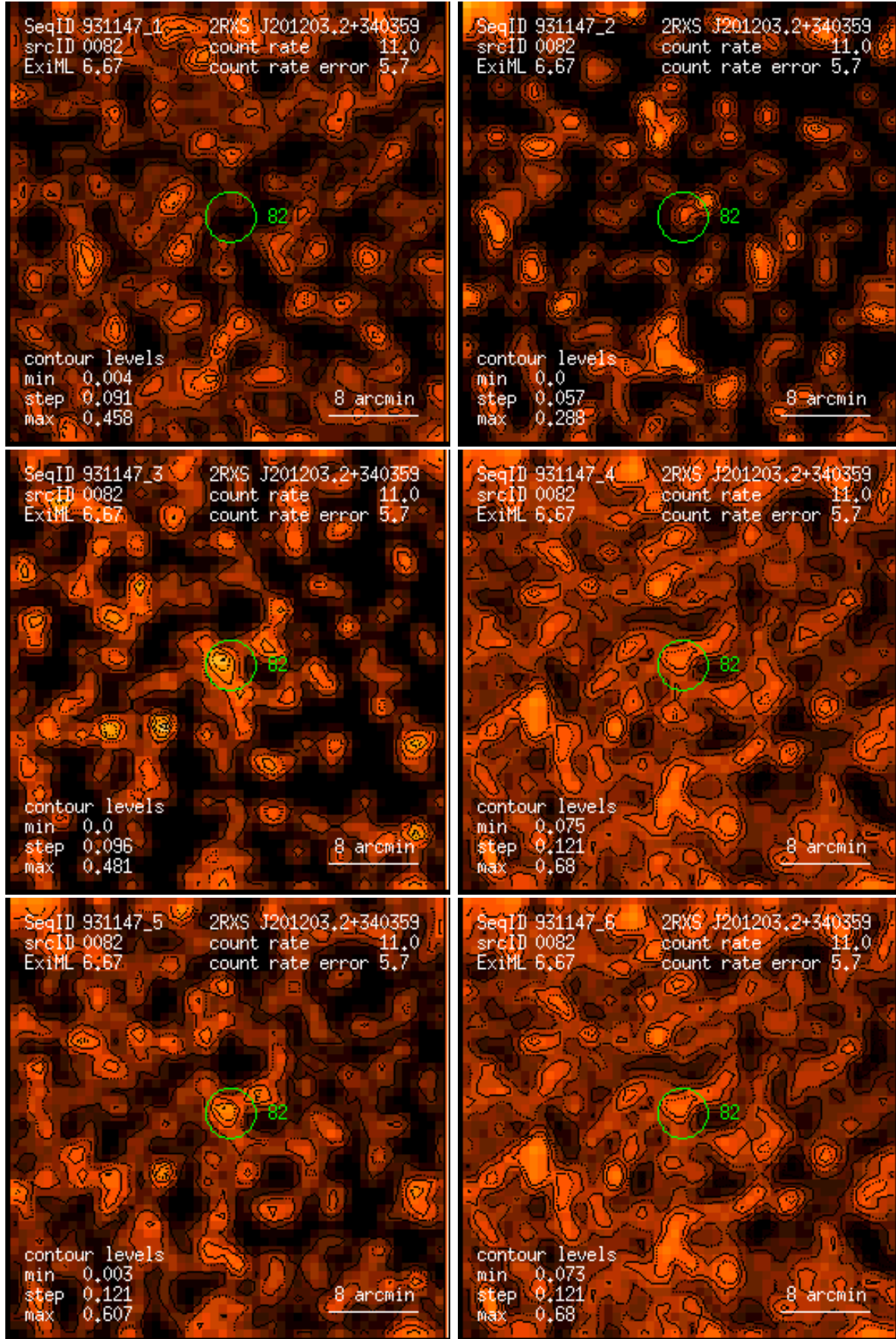
Figure 82: RASS 931147: detection 0082: band rate images, Gaussian filter: (1) PSPC channels 11 – 41, (2) 52 – 90, (3) 91 – 201, (4) 11 – 235, (5) 52 – 201, (6) 11 – 201. Broad band rates in counts/ks. Band rate contour levels in counts/ks/arcmin 2 .
